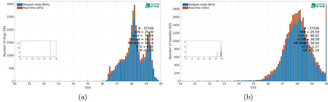
Figure 3: Histograms of SSS from Argo (a) and SMOS SSS L4 v2 - Daily (BEC) (b) considering all match-up pairs per bins of 0.1 over the Mediterranean Sea Pi-MEP region and for the full satellite product period.
