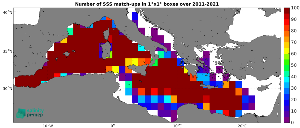
Figure 5: Number of SSS match-ups between Argo SSS and the SMOS SSS L4 v2 - Daily (BEC) SSS product for the Mediterranean Sea Pi-MEP region over 1^\circ \times 1^\circ boxes and for the full satellite product period.
