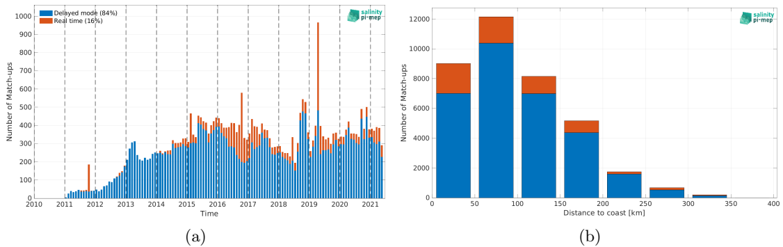
Figure 2: Number of match-ups between Argo and SMOS SSS L4 v2 - Daily (BEC) SSS as a function of time (a) and as function of the distance to coast (b) over the Mediterranean Sea Pi-MEP region and for the full satellite product period.
