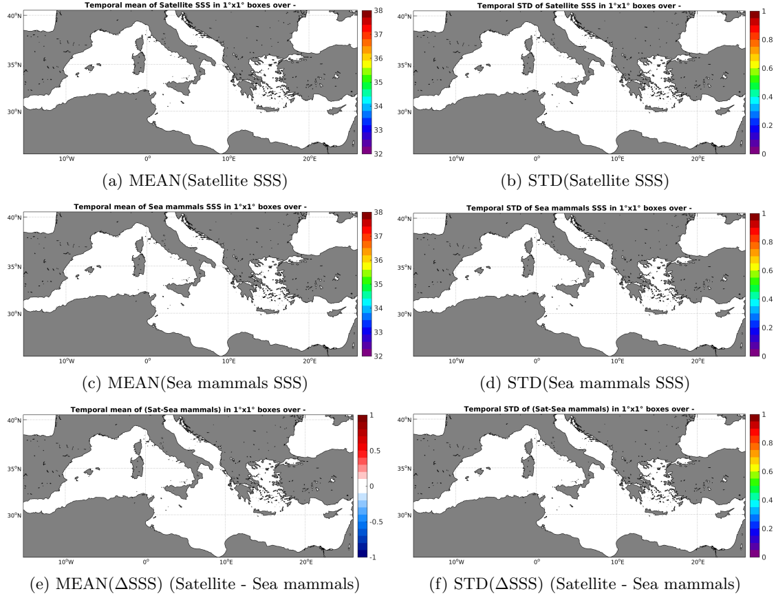
Figure 6: Temporal mean (left) and STD (right) of SSS from SMOS-L3-ICDC-V3-MONTHLY-0.5DEG (top), Sea mammals (middle), and of \Delta SSS (Satellite - Sea mammals). Only match-up pairs are used to generate these maps.
