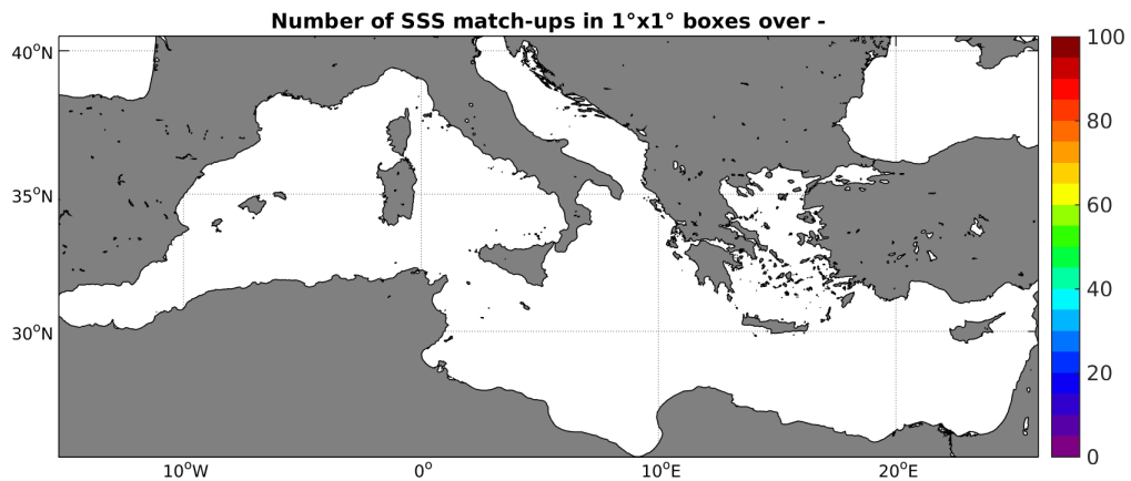
Figure 4: Number of SSS match-ups between Sea mammals SSS and the SMOS-L3-ICDC-V3-MONTHLY-0.5DEG SSS product for the Mediterranean Sea Pi-MEP region over 1^\circ \times 1^\circ boxes and for the full satellite product period.
