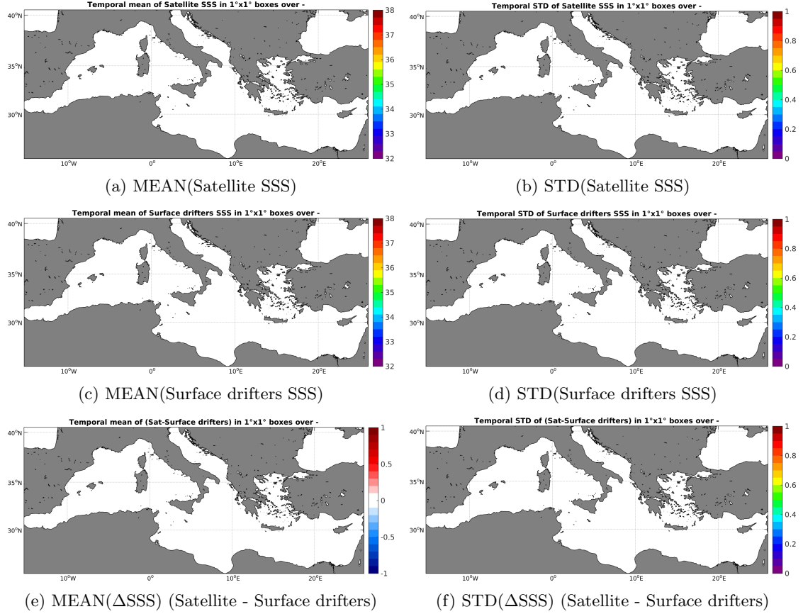
Figure 5: Temporal mean (left) and STD (right) of SSS from SMOS-L3-ICDC-V3-MONTHLY-0.5DEG (top), Surface drifters (middle), and of \Delta\text{SSS} (Satellite - Surface drifters). Only match-up pairs are used to generate these maps.
