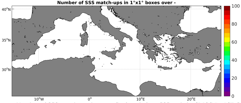
Figure 3: Number of SSS match-ups between Surface drifters SSS and the SMOS-L3-ICDC-V3-MONTHLY-0.5DEG SSS product for the Mediterranean Sea Pi-MEP region over 1^\circ \times 1^\circ boxes and for the full satellite product period.
