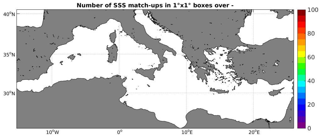
Figure 4: Number of SSS match-ups between Argo SSS and the SMOS-L3-ICDC-V3-MONTHLY-0.5DEG SSS product for the Mediterranean Sea Pi-MEP region over 1^\circ \times 1^\circ boxes and for the full satellite product period.
