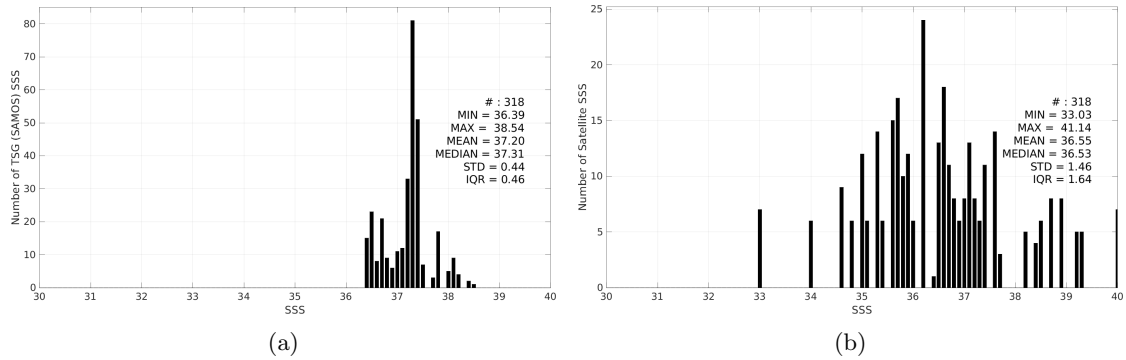
Figure 3: Histograms of SSS from TSG (SAMOS) (a) and SMOS SSS L2Q v331 - With FLAG (CMEMS-CATDS-CPDC) (b) considering all match-up pairs per bins of 0.1 over the Mediterranean Sea Pi-MEP region and for the full satellite product period.
