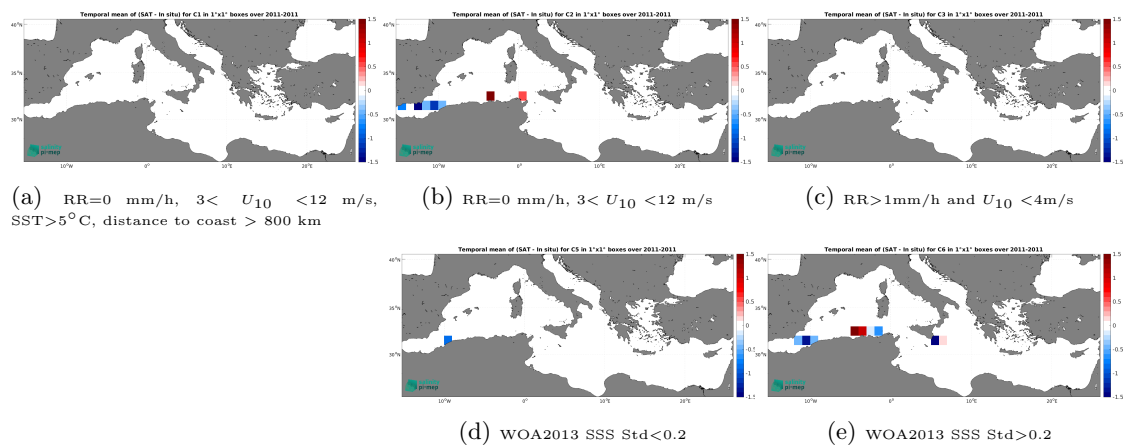
Figure 14: Temporal mean gridded over spatial boxes of size 1^\circ \times 1^\circ of \Delta SSS (SMOS SSS L2Q v331 - With FLAG (CMEMS-CATDS-CPDC) - TSG (SAMOS)) for 5 different subdatasets corresponding to:RR=0 mm/h, 3 < U_{10} < 12 m/s, SST>5°C, distance to coast > 800 km (a), RR=0 mm/h, 3 < U_{10} < 12 m/s (b), RR>1mm/h and U_{10} < 4 m/s (c), WOA2013 SSS Std<0.2 (d), WOA2013 SSS Std>0.2 (e).
