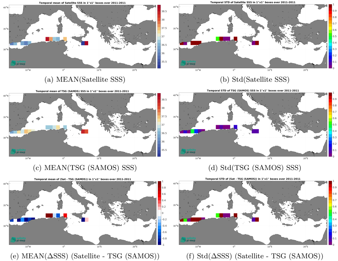
Figure 7: Temporal mean (left) and Std (right) of SSS from SMOS SSS L2Q v331 - With FLAG (CMEMS-CATDS-CPDC) (top), TSG (SAMOS) (middle), and of \Delta\text{SSS} (Satellite - TSG (SAMOS)). Only match-up pairs are used to generate these maps.
