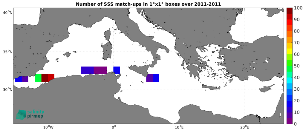
Figure 5: Number of SSS match-ups between TSG (SAMOS) SSS and the SMOS SSS L2Q v331 - With FLAG (CMEMS-CATDS-CPDC) SSS product for the Mediterranean Sea Pi-MEP region over 1^\circ \times 1^\circ boxes and for the full satellite product period.
