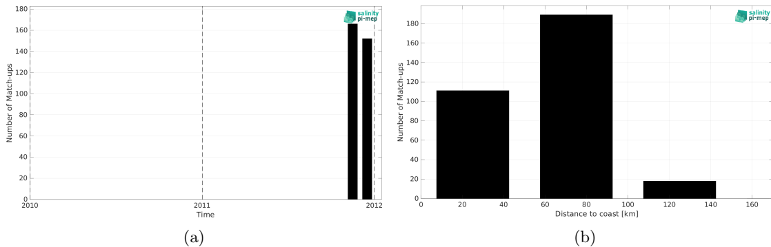
Figure 2: Number of match-ups between TSG (SAMOS) and SMOS SSS L2Q v331 - With FLAG (CMEMS-CATDS-CPDC) SSS as a function of time (a) and as function of the distance to coast (b) over the Mediterranean Sea Pi-MEP region and for the full satellite product period.
