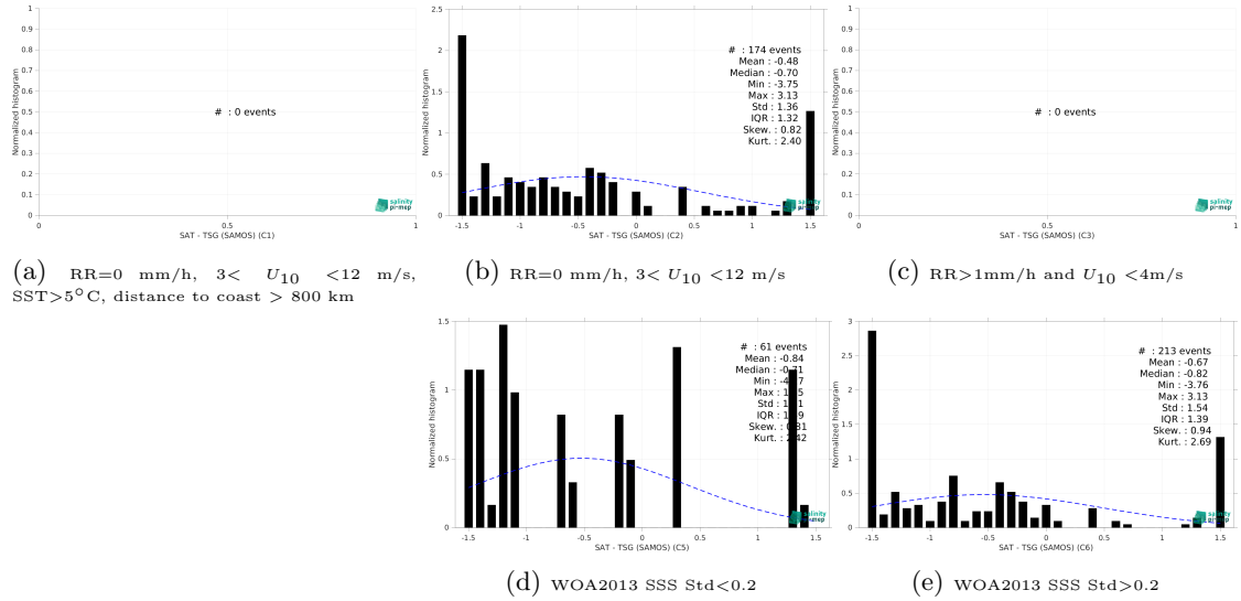
Figure 15: Normalized histogram of \Delta SSS (SMOS SSS L2Q v331 - With FLAG (CMEMS-CATDS-CPDC) - TSG (SAMOS)) for 5 different subdatasets corresponding to: RR=0 mm/h, 3 < U_{10} < 12 m/s, SST>5°C, distance to coast > 800 km (a), RR=0 mm/h, 3 < U_{10} < 12 m/s (b), RR>1mm/h and U_{10} < 4 m/s (c), WOA2013 SSS Std<0.2 (d), WOA2013 SSS Std>0.2 (e).
