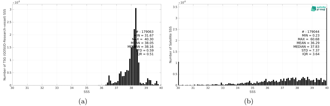
Figure 2: Histograms of SSS from TSG (GOSUD-Research-vessel) (a) and SMOS SSS L2Q v331 - With FLAG (CMEMS-CATDS-CPDC) (b) considering all match-up pairs per bins of 0.1 over the Mediterranean Sea Pi-MEP region and for the full satellite product period.
