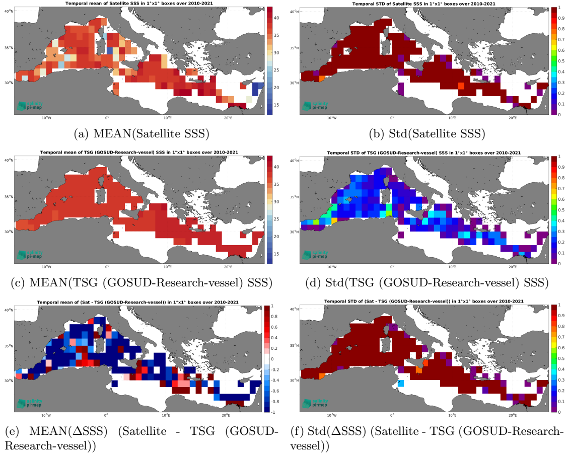
Figure 6: Temporal mean (left) and Std (right) of SSS from SMOS SSS L2Q v331 - With FLAG (CMEMS-CATDS-CPDC) (top), TSG (GOSUD-Research-vessel) (middle), and of \Delta\text{SSS} (Satellite - TSG (GOSUD-Research-vessel)). Only match-up pairs are used to generate these maps.
