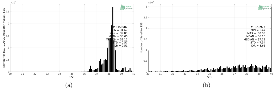
Figure 2: Histograms of SSS from TSG (GOSUD-Research-vessel) (a) and SMOS SSS L2Q v331 - With FLAG (CMEMS-CATDS-CPDC) (b) considering all match-up pairs per bins of 0.1 over the Mediterranean Sea Pi-MEP region and for the full satellite product period.
