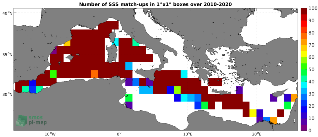
Figure 4: Number of SSS match-ups between TSG (GOSUD-Research-vessel) SSS and the SMOS SSS L2Q v331 - With FLAG (CMEMS-CATDS-CPDC) SSS product for the Mediterranean Sea Pi-MEP region over 1^\circ \times 1^\circ boxes and for the full satellite product period.
