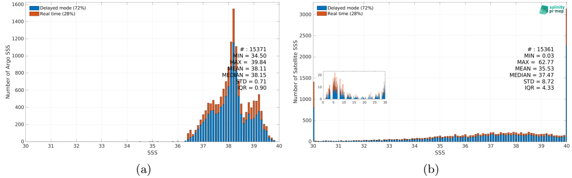
Figure 3: Histograms of SSS from Argo (a) and SMOS SSS L2Q v331 - With FLAG (CMEMS-CATDS-CPDC) (b) considering all match-up pairs per bins of 0.1 over the Mediterranean Sea Pi-MEP region and for the full satellite product period.
