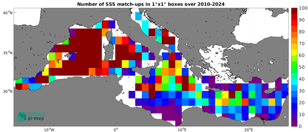
Figure 5: Number of SSS match-ups between Argo SSS and the SMOS SSS L2Q v331 - With FLAG (CMEMS-CATDS-CPDC) SSS product for the Mediterranean Sea Pi-MEP region over 1^\circ \times 1^\circ boxes and for the full satellite product period.
