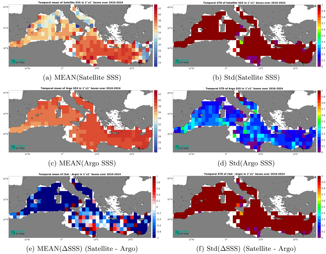
Figure 7: Temporal mean (left) and Std (right) of SSS from SMOS SSS L2Q v331 - With FLAG (CMEMS-CATDS-CPDC) (top), Argo (middle), and of \Delta\text{SSS} (Satellite - Argo). Only match-up pairs are used to generate these maps.
