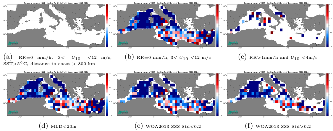
Figure 14: Temporal mean gridded over spatial boxes of size 1^\circ \times 1^\circ of \Delta SSS (SMOS SSS L2Q v331 - With FLAG (CMEMS-CATDS-CPDC) - Argo) for 6 different subdatasets corresponding to:RR=0 mm/h, 3 < U_{10} < 12 m/s, SST >5^\circ C, distance to coast > 800 km (a), RR=0 mm/h, 3 < U_{10} < 12 m/s (b), RR >1 mm/h and U_{10} < 4 m/s (c),MLD <20 m (d),WOA2013 SSS Std <0.2 (e),WOA2013 SSS Std >0.2 (f).
