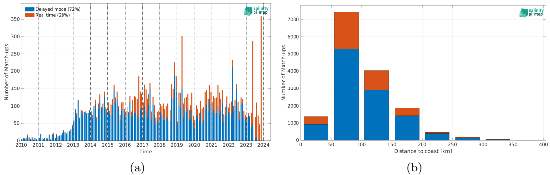
Figure 2: Number of match-ups between Argo and SMOS SSS L2Q v331 - With FLAG (CMEMS-CATDS-CPDC) SSS as a function of time (a) and as function of the distance to coast (b) over the Mediterranean Sea Pi-MEP region and for the full satellite product period.
