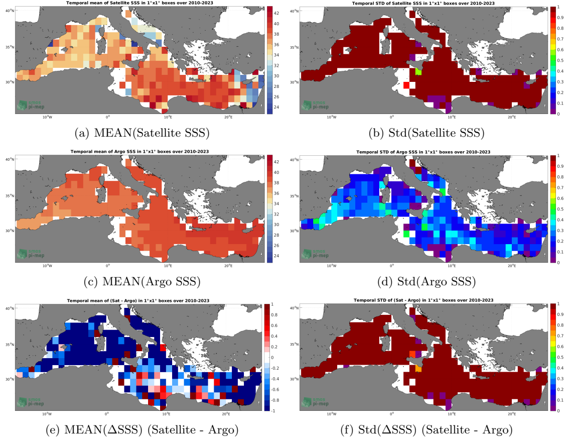
Figure 6: Temporal mean (left) and Std (right) of SSS from SMOS SSS L2Q v331 - With FLAG (CMEMS-CATDS-CPDC) (top), Argo (middle), and of \Delta\text{SSS} (Satellite - Argo). Only match-up pairs are used to generate these maps.
