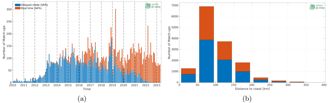
Figure 1: Number of match-ups between Argo and SMOS SSS L2Q v331 - With FLAG (CMEMS-CATDS-CPDC) SSS as a function of time (a) and as function of the distance to coast (b) over the Mediterranean Sea Pi-MEP region and for the full satellite product period.
