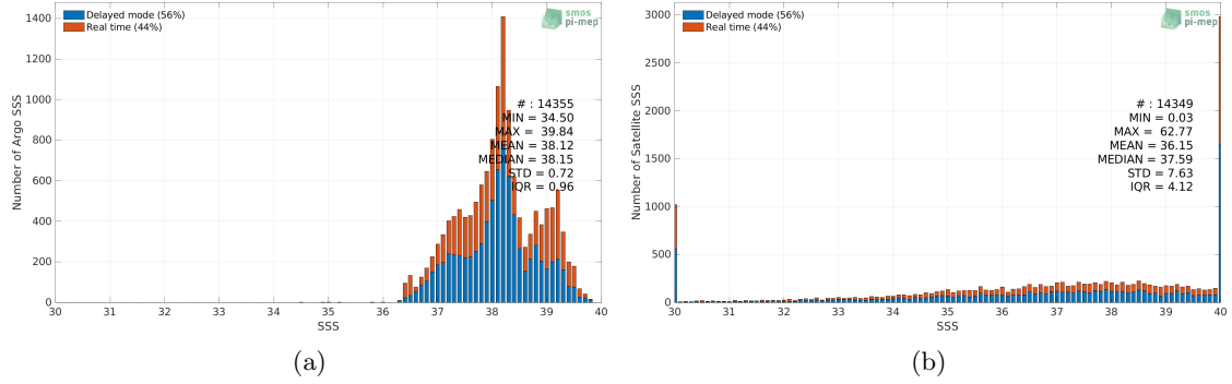
Figure 2: Histograms of SSS from Argo (a) and SMOS SSS L2Q v331 - With FLAG (CMEMS-CATDS-CPDC) (b) considering all match-up pairs per bins of 0.1 over the Mediterranean Sea Pi-MEP region and for the full satellite product period.
