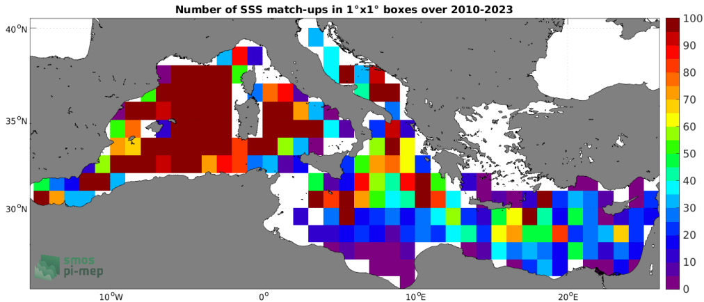
Figure 4: Number of SSS match-ups between Argo SSS and the SMOS SSS L2Q v331 - With FLAG (CMEMS-CATDS-CPDC) SSS product for the Mediterranean Sea Pi-MEP region over 1^\circ \times 1^\circ boxes and for the full satellite product period.
