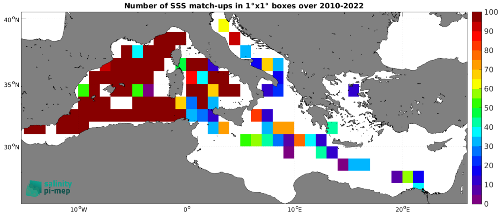
Figure 5: Number of SSS match-ups between TSG (LEGOS-DM) SSS and the SMOS SSS L2Q v331 - No FLAG (CMEMS-CATDS-CPDC) SSS product for the Mediterranean Sea Pi-MEP region over 1^\circ \times 1^\circ boxes and for the full satellite product period.
