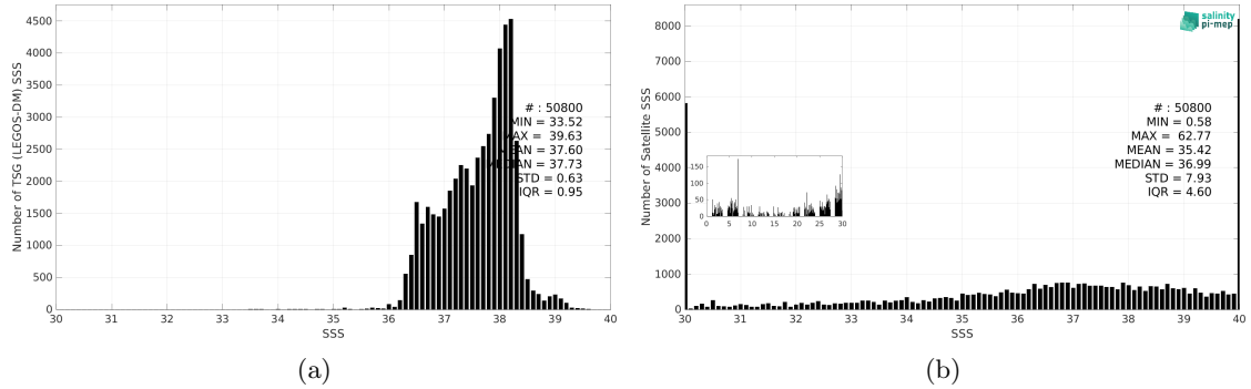
Figure 3: Histograms of SSS from TSG (LEGOS-DM) (a) and SMOS SSS L2Q v331 - No FLAG (CMEMS-CATDS-CPDC) (b) considering all match-up pairs per bins of 0.1 over the Mediterranean Sea Pi-MEP region and for the full satellite product period.
