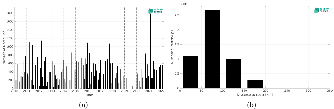
Figure 2: Number of match-ups between TSG (LEGOS-DM) and SMOS SSS L2Q v331 - No FLAG (CMEMS-CATDS-CPDC) SSS as a function of time (a) and as function of the distance to coast (b) over the Mediterranean Sea Pi-MEP region and for the full satellite product period.
