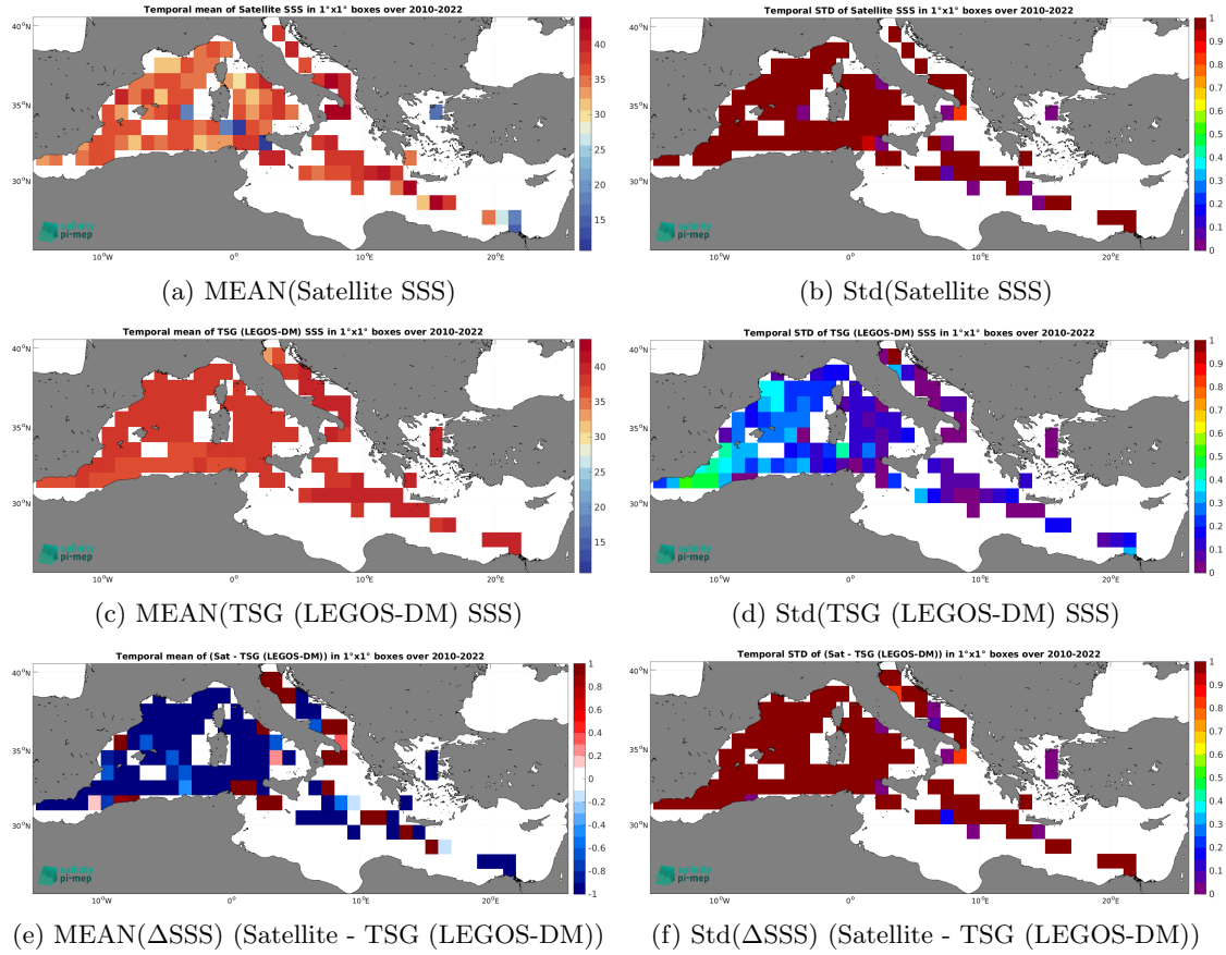
Figure 7: Temporal mean (left) and Std (right) of SSS from SMOS SSS L2Q v331 - No FLAG (CMEMS-CATDS-CPDC) (top), TSG (LEGOS-DM) (middle), and of \Delta\text{SSS} (Satellite - TSG (LEGOS-DM)). Only match-up pairs are used to generate these maps.
