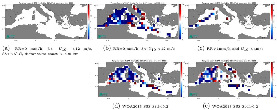
Figure 14: Temporal mean gridded over spatial boxes of size 1^\circ \times 1^\circ of \Delta SSS (SMOS SSS L2Q v331 - No FLAG (CMEMS-CATDS-CPDC) - TSG (LEGOS-DM)) for 5 different subdatasets corresponding to: RR=0 mm/h, 3 < U_{10} < 12 m/s, SST>5°C, distance to coast > 800 km (a), RR=0 mm/h, 3 < U_{10} < 12 m/s (b), RR>1mm/h and U_{10} < 4 m/s (c), WOA2013 SSS Std<0.2 (d), WOA2013 SSS Std>0.2 (e).
