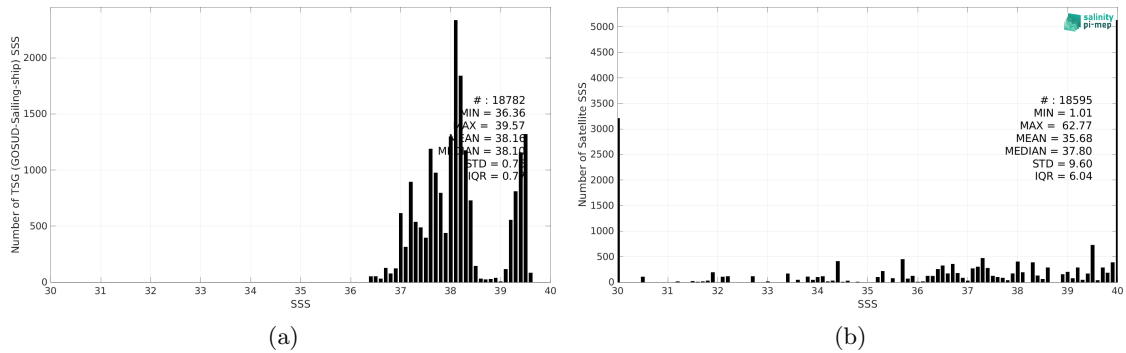
Figure 2: Histograms of SSS from TSG (GOSUD-Sailing-ship) (a) and SMOS SSS L2Q v331 - No FLAG (CMEMS-CATDS-CPDC) (b) considering all match-up pairs per bins of 0.1 over the Mediterranean Sea Pi-MEP region and for the full satellite product period.
