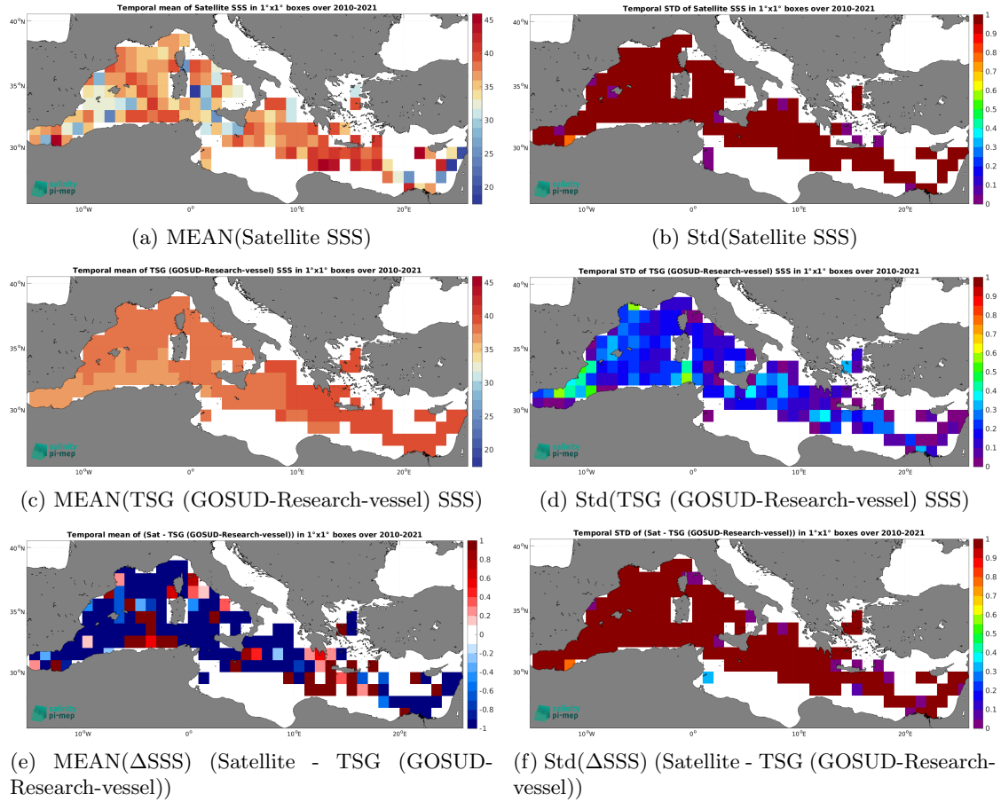
Figure 6: Temporal mean (left) and Std (right) of SSS from SMOS SSS L2Q v331 - No FLAG (CMEMS-CATDS-CPDC) (top), TSG (GOSUD-Research-vessel) (middle), and of \Delta\text{SSS} (Satellite - TSG (GOSUD-Research-vessel)). Only match-up pairs are used to generate these maps.
