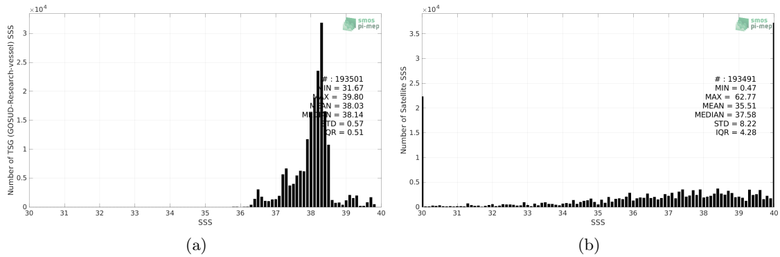
Figure 2: Histograms of SSS from TSG (GOSUD-Research-vessel) (a) and SMOS SSS L2Q v331 - No FLAG (CMEMS-CATDS-CPDC) (b) considering all match-up pairs per bins of 0.1 over the Mediterranean Sea Pi-MEP region and for the full satellite product period.
