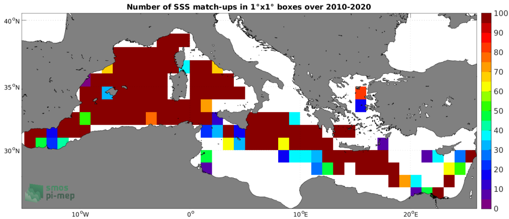
Figure 4: Number of SSS match-ups between TSG (GOSUD-Research-vessel) SSS and the SMOS SSS L2Q v331 - No FLAG (CMEMS-CATDS-CPDC) SSS product for the Mediterranean Sea Pi-MEP region over 1^\circ \times 1^\circ boxes and for the full satellite product period.
