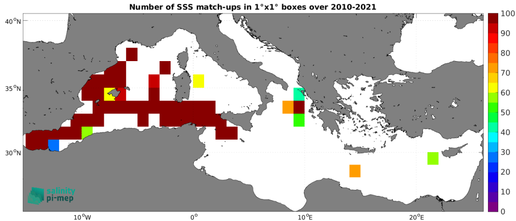
Figure 4: Number of SSS match-ups between TSG (CSIC-UTM) SSS and the SMOS SSS L2Q v331 - No FLAG (CMEMS-CATDS-CPDC) SSS product for the Mediterranean Sea Pi-MEP region over 1^\circ \times 1^\circ boxes and for the full satellite product period.
