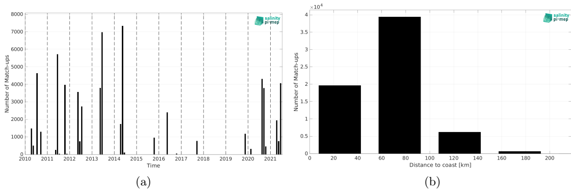
Figure 1: Number of match-ups between TSG (CSIC-UTM) and SMOS SSS L2Q v331 - No FLAG (CMEMS-CATDS-CPDC) SSS as a function of time (a) and as function of the distance to coast (b) over the Mediterranean Sea Pi-MEP region and for the full satellite product period.
