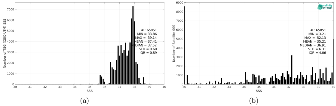
Figure 2: Histograms of SSS from TSG (CSIC-UTM) (a) and SMOS SSS L2Q v331 - No FLAG (CMEMS-CATDS-CPDC) (b) considering all match-up pairs per bins of 0.1 over the Mediterranean Sea Pi-MEP region and for the full satellite product period.
