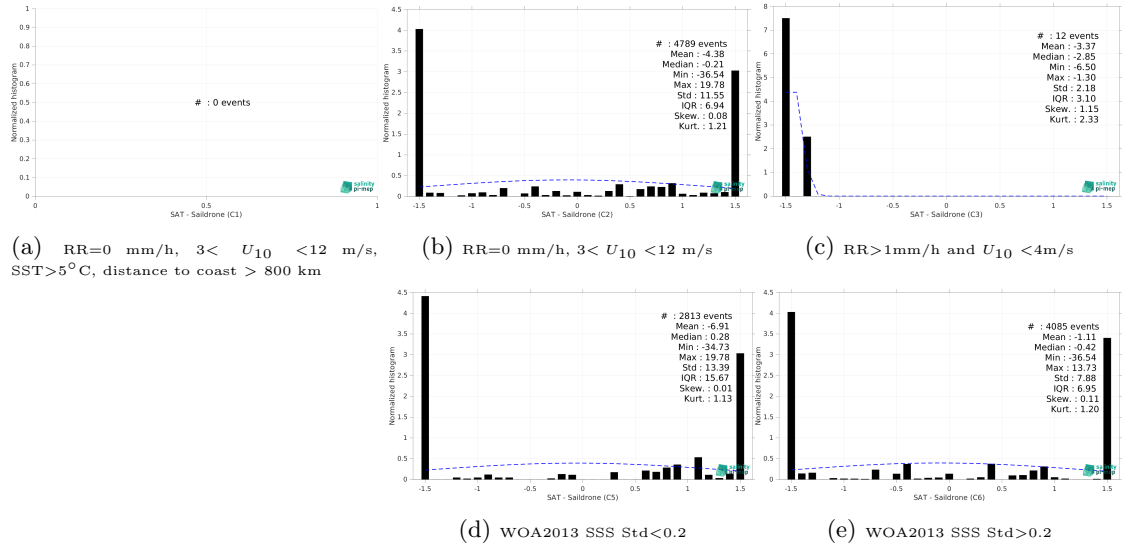
Figure 15: Normalized histogram of \Delta SSS (SMOS SSS L2Q v331 - No FLAG (CMEMS-CATDS-CPDC) - Saldrone) for 5 different subdatasets corresponding to: RR=0 mm/h, 3 < U_{10} < 12 m/s, SST > 5°C, distance to coast > 800 km (a), RR=0 mm/h, 3 < U_{10} < 12 m/s (b), RR > 1mm/h and U_{10} < 4 m/s (c), WOA2013 SSS Std < 0.2 (d), WOA2013 SSS Std > 0.2 (e).
