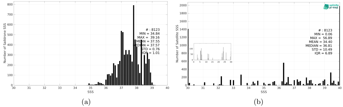
Figure 3: Histograms of SSS from Saildrone (a) and SMOS SSS L2Q v331 - No FLAG (CMEMS-CATDS-CPDC) (b) considering all match-up pairs per bins of 0.1 over the Mediterranean Sea Pi-MEP region and for the full satellite product period.
