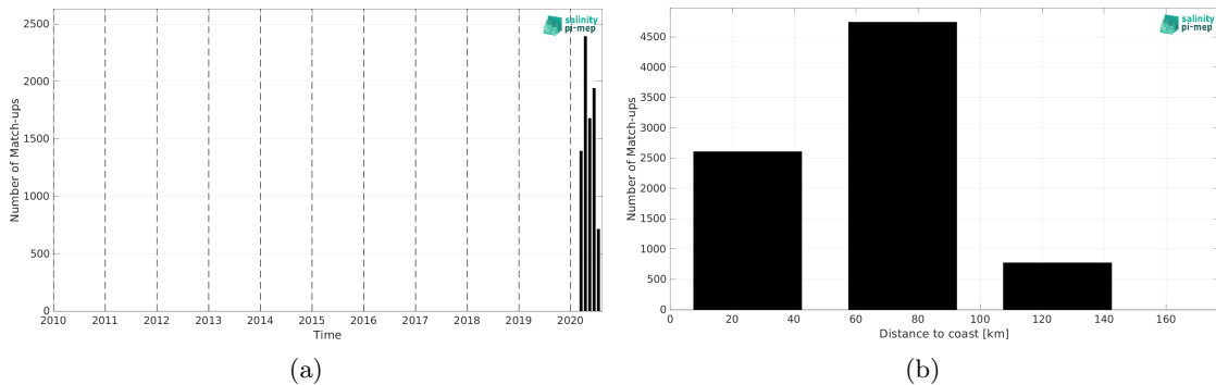
Figure 2: Number of match-ups between Saildrone and SMOS SSS L2Q v331 - No FLAG (CMEMS-CATDS-CPDC) SSS as a function of time (a) and as function of the distance to coast (b) over the Mediterranean Sea Pi-MEP region and for the full satellite product period.
