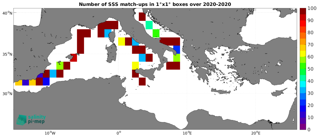
Figure 5: Number of SSS match-ups between Saildrone SSS and the SMOS SSS L2Q v331 - No FLAG (CMEMS-CATDS-CPDC) SSS product for the Mediterranean Sea Pi-MEP region over 1^\circ \times 1^\circ boxes and for the full satellite product period.
