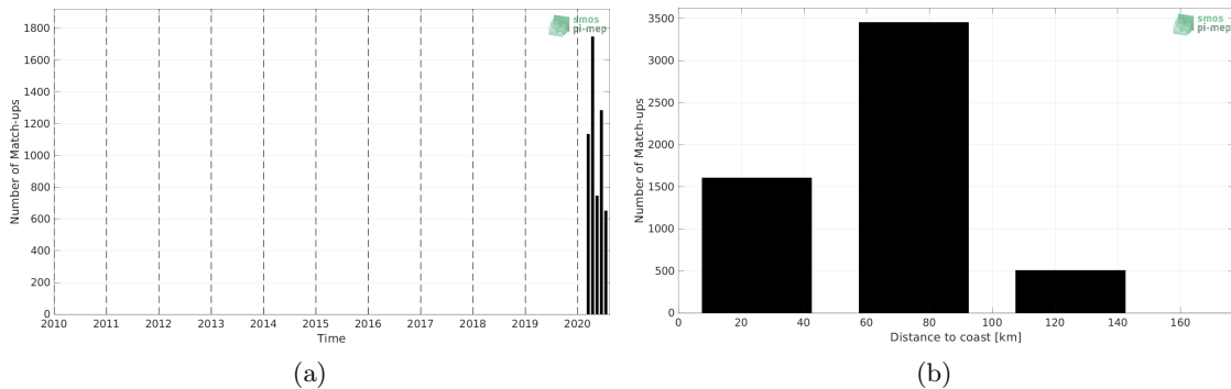
Figure 1: Number of match-ups between Saildrone and SMOS SSS L2Q v331 - No FLAG (CMEMS-CATDS-CPDC) SSS as a function of time (a) and as function of the distance to coast (b) over the Mediterranean Sea Pi-MEP region and for the full satellite product period.
