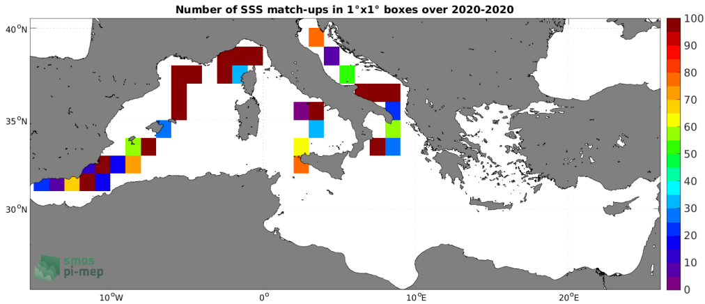
Figure 4: Number of SSS match-ups between Saildrone SSS and the SMOS SSS L2Q v331 - No FLAG (CMEMS-CATDS-CPDC) SSS product for the Mediterranean Sea Pi-MEP region over 1^\circ \times 1^\circ boxes and for the full satellite product period.
