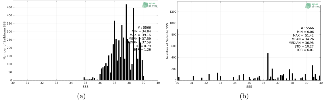
Figure 2: Histograms of SSS from Saildrone (a) and SMOS SSS L2Q v331 - No FLAG (CMEMS-CATDS-CPDC) (b) considering all match-up pairs per bins of 0.1 over the Mediterranean Sea Pi-MEP region and for the full satellite product period.
