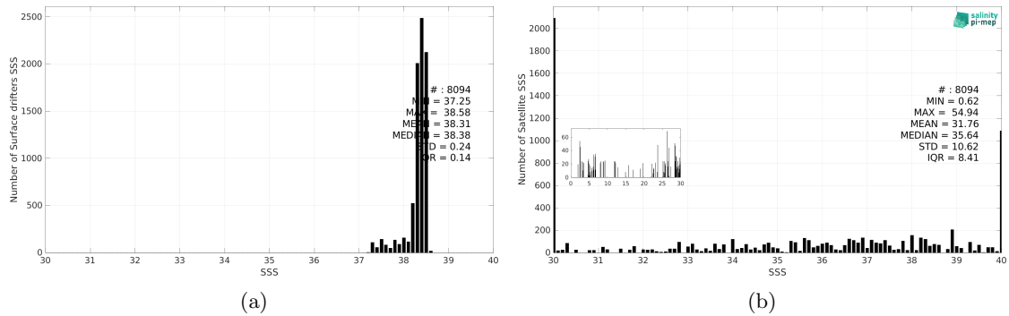
Figure 3: Histograms of SSS from Surface drifters (a) and SMOS SSS L2Q v331 - No FLAG (CMEMS-CATDS-CPDC) (b) considering all match-up pairs per bins of 0.1 over the Mediterranean Sea Pi-MEP region and for the full satellite product period.
