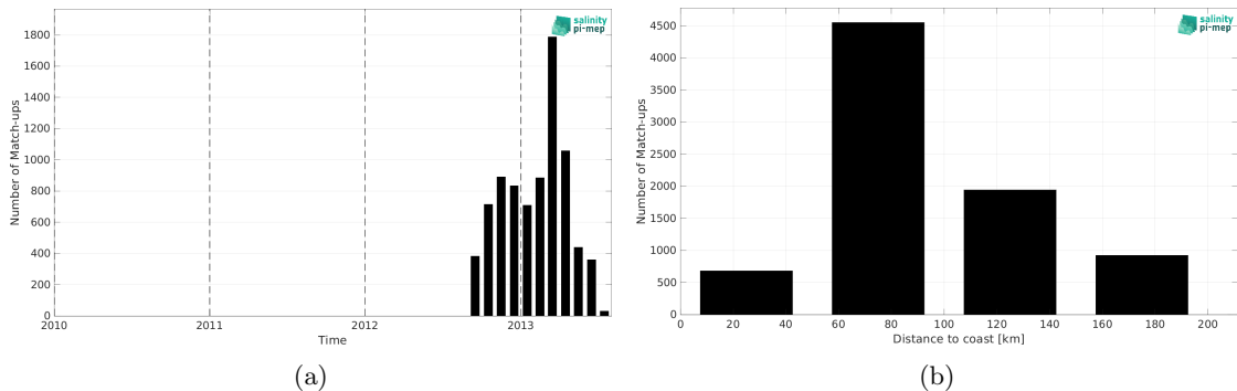
Figure 2: Number of match-ups between Surface drifters and SMOS SSS L2Q v331 - No FLAG (CMEMS-CATDS-CPDC) SSS as a function of time (a) and as function of the distance to coast (b) over the Mediterranean Sea Pi-MEP region and for the full satellite product period.
