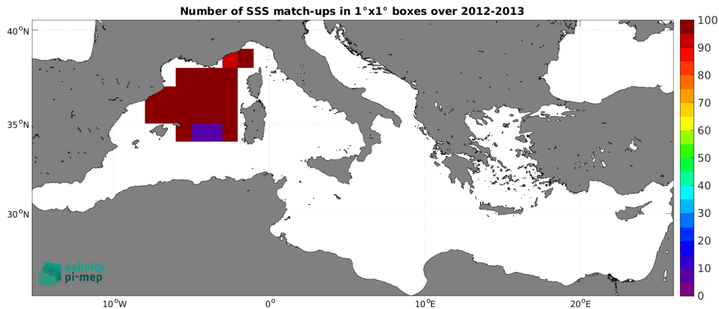
Figure 4: Number of SSS match-ups between Surface drifters SSS and the SMOS SSS L2Q v331 - No FLAG (CMEMS-CATDS-CPDC) SSS product for the Mediterranean Sea Pi-MEP region over 1^\circ \times 1^\circ boxes and for the full satellite product period.
