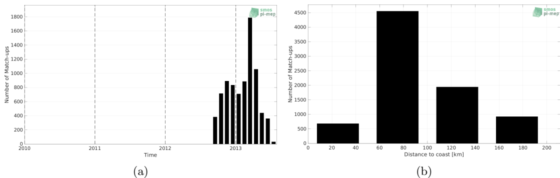
Figure 1: Number of match-ups between Surface drifters and SMOS SSS L2Q v331 - No FLAG (CMEMS-CATDS-CPDC) SSS as a function of time (a) and as function of the distance to coast (b) over the Mediterranean Sea Pi-MEP region and for the full satellite product period.
