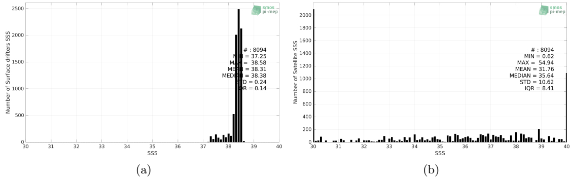
Figure 2: Histograms of SSS from Surface drifters (a) and SMOS SSS L2Q v331 - No FLAG (CMEMS-CATDS-CPDC) (b) considering all match-up pairs per bins of 0.1 over the Mediterranean Sea Pi-MEP region and for the full satellite product period.
