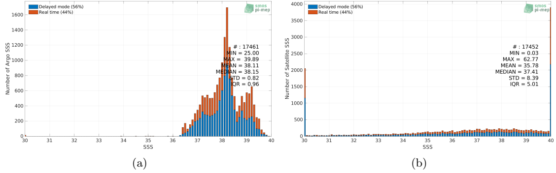
Figure 2: Histograms of SSS from Argo (a) and SMOS SSS L2Q v331 - No FLAG (CMEMS-CATDS-CPDC) (b) considering all match-up pairs per bins of 0.1 over the Mediterranean Sea Pi-MEP region and for the full satellite product period.
