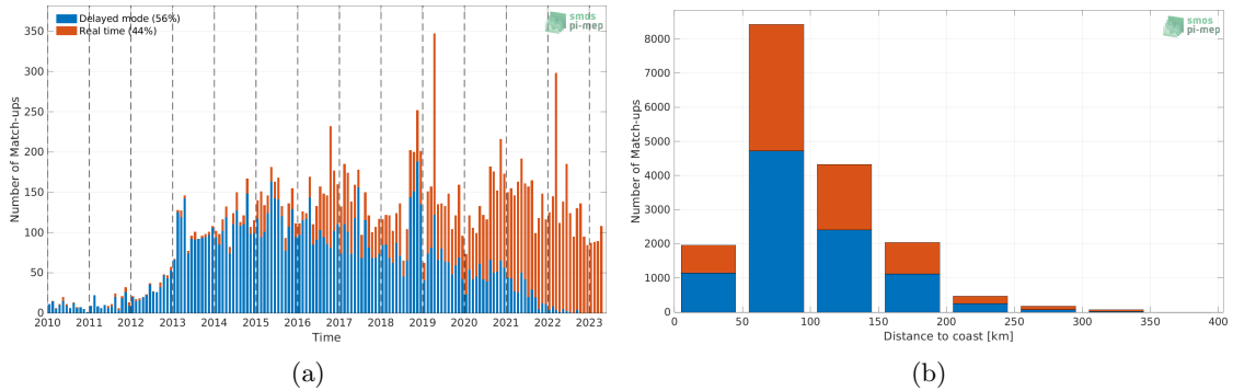
Figure 1: Number of match-ups between Argo and SMOS SSS L2Q v331 - No FLAG (CMEMS-CATDS-CPDC) SSS as a function of time (a) and as function of the distance to coast (b) over the Mediterranean Sea Pi-MEP region and for the full satellite product period.
