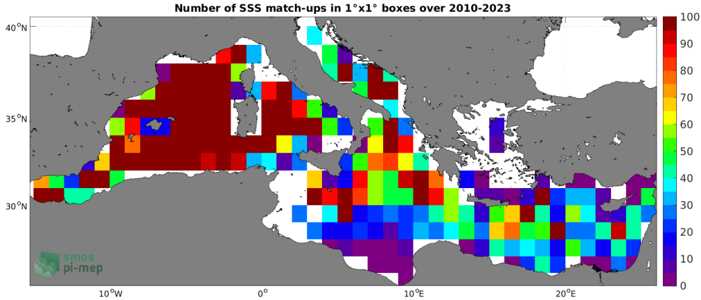
Figure 4: Number of SSS match-ups between Argo SSS and the SMOS SSS L2Q v331 - No FLAG (CMEMS-CATDS-CPDC) SSS product for the Mediterranean Sea Pi-MEP region over 1^\circ \times 1^\circ boxes and for the full satellite product period.
