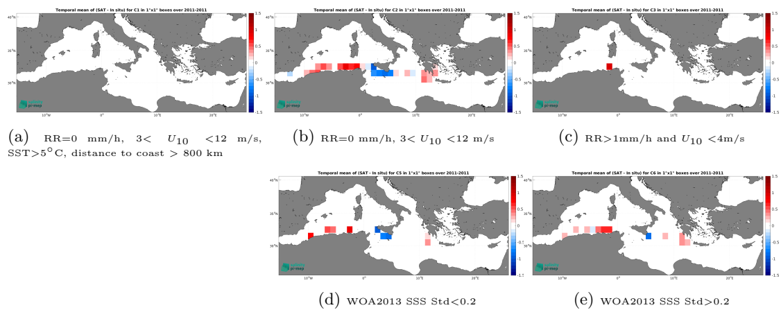
Figure 14: Temporal mean gridded over spatial boxes of size 1^\circ \times 1^\circ of \Delta\text{SSS} (SMOS SSS L3 v9 - 9 Days (CATDS-CEC-LOCEAN) - TSG (SAMOS)) for 5 different subdatasets corresponding to:RR=0 mm/h, 3 < U_{10} < 12 m/s, SST>5°C, distance to coast > 800 km (a), RR=0 mm/h, 3 < U_{10} < 12 m/s (b), RR>1mm/h and U_{10} < 4 m/s (c), WOA2013 SSS Std<0.2 (d), WOA2013 SSS Std>0.2 (e).
