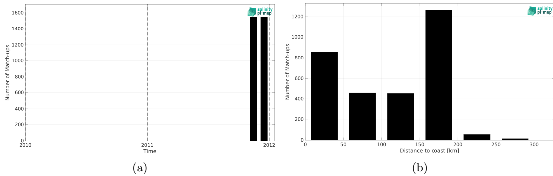
Figure 2: Number of match-ups between TSG (SAMOS) and SMOS SSS L3 v9 - 9 Days (CATDS-CEC-LOCEAN) SSS as a function of time (a) and as function of the distance to coast (b) over the Mediterranean Sea Pi-MEP region and for the full satellite product period.
