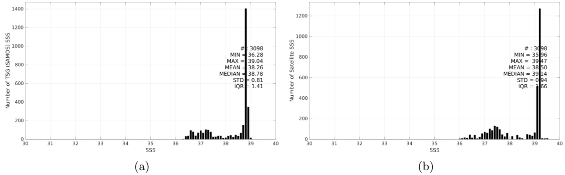
Figure 3: Histograms of SSS from TSG (SAMOS) (a) and SMOS SSS L3 v9 - 9 Days (CATDS-CEC-LOCEAN) (b) considering all match-up pairs per bins of 0.1 over the Mediterranean Sea Pi-MEP region and for the full satellite product period.
