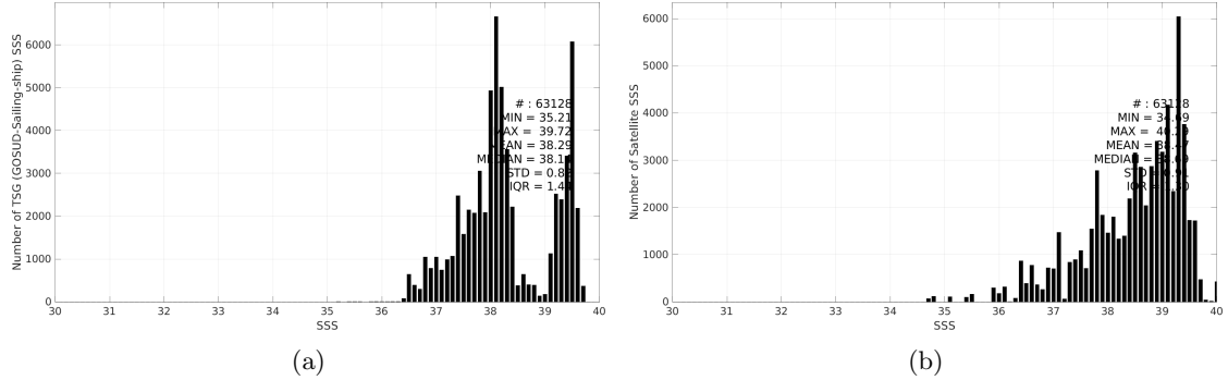
Figure 3: Histograms of SSS from TSG (GOSUD-Sailing-ship) (a) and SMOS SSS L3 v9 - 9 Days (CATDS-CEC-LOCEAN) (b) considering all match-up pairs per bins of 0.1 over the Mediterranean Sea Pi-MEP region and for the full satellite product period.
