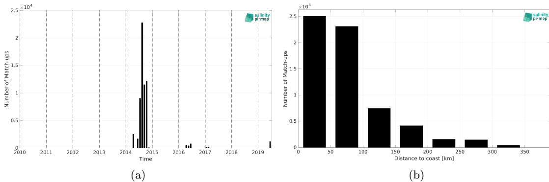
Figure 2: Number of match-ups between TSG (GOSUD-Sailing-ship) and SMOS SSS L3 v9 - 9 Days (CATDS-CEC-LOCEAN) SSS as a function of time (a) and as function of the distance to coast (b) over the Mediterranean Sea Pi-MEP region and for the full satellite product period.
