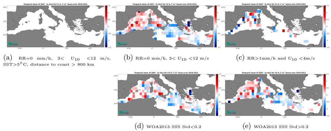
Figure 14: Temporal mean gridded over spatial boxes of size 1^\circ \times 1^\circ of \Delta SSS (SMOS SSS L3 v9 - 9 Days (CATDS-CEC-LOCEAN) - TSG (GOSUD-Research-vessel)) for 5 different subdatasets corresponding to:RR=0 mm/h, 3 < U_{10} < 12 m/s, SST>5°C, distance to coast > 800 km (a), RR=0 mm/h, 3 < U_{10} < 12 m/s (b), RR>1mm/h and U_{10} < 4 m/s (c), WOA2013 SSS Std<0.2 (d), WOA2013 SSS Std>0.2 (e).
