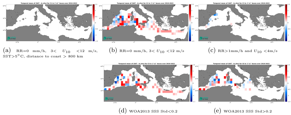
Figure 14: Temporal mean gridded over spatial boxes of size 1^\circ \times 1^\circ of \Delta SSS (SMOS SSS L3 v9 - 9 Days (CATDS-CEC-LOCEAN) - TSG (CSIC-UTM)) for 5 different subdatasets corresponding to:RR=0 mm/h, 3 < U_{10} < 12 m/s, SST >5^\circ C, distance to coast > 800 km (a), RR=0 mm/h, 3 < U_{10} < 12 m/s (b), RR >1 mm/h and U_{10} < 4 m/s (c), WOA2013 SSS Std <0.2 (d), WOA2013 SSS Std >0.2 (e).
