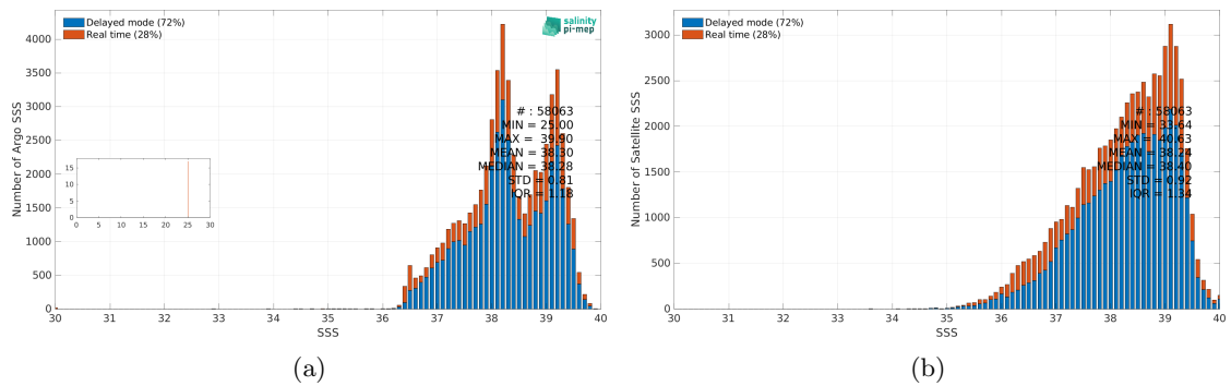
Figure 3: Histograms of SSS from Argo (a) and SMOS SSS L3 v9 - 9 Days (CATDS-CEC-LOCEAN) (b) considering all match-up pairs per bins of 0.1 over the Mediterranean Sea Pi-MEP region and for the full satellite product period.
