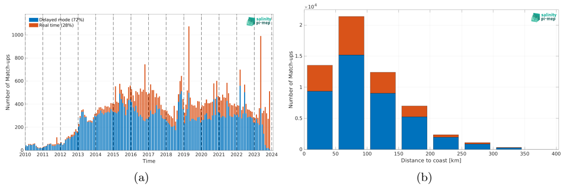
Figure 2: Number of match-ups between Argo and SMOS SSS L3 v9 - 9 Days (CATDS-CEC-LOCEAN) SSS as a function of time (a) and as function of the distance to coast (b) over the Mediterranean Sea Pi-MEP region and for the full satellite product period.
