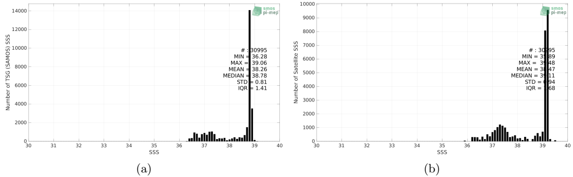
Figure 2: Histograms of SSS from TSG (SAMOS) (a) and SMOS SSS L3 v8 - 9 Days (CATDS-CECOS-LOCEAN) (b) considering all match-up pairs per bins of 0.1 over the Mediterranean Sea Pi-MEP region and for the full satellite product period.
