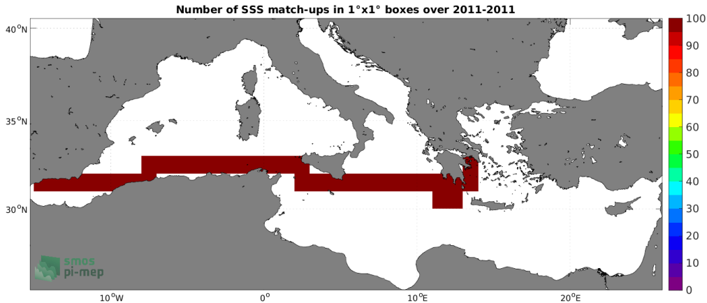
Figure 4: Number of SSS match-ups between TSG (SAMOS) SSS and the SMOS SSS L3 v8 - 9 Days (CATDS-CECOS-LOCEAN) SSS product for the Mediterranean Sea Pi-MEP region over 1^\circ \times 1^\circ boxes and for the full satellite product period.
