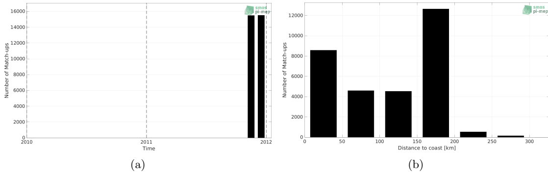
Figure 1: Number of match-ups between TSG (SAMOS) and SMOS SSS L3 v8 - 9 Days (CATDS-CECOS-LOCEAN) SSS as a function of time (a) and as function of the distance to coast (b) over the Mediterranean Sea Pi-MEP region and for the full satellite product period.
