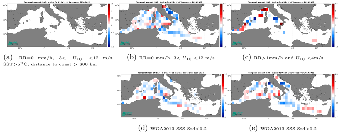
Figure 12: Temporal mean gridded over spatial boxes of size 1^{\circ}\times 1^{\circ} of \Delta\text{SSS} (SMOS SSS L3 v8 - 9 Days (CATDS-CEC-LOCEAN) - TSG (LEGOS-DM)) for 5 different subdatasets corresponding to:RR=0 mm/h, 3 < U_{10} < 12 m/s, SST > 5^{\circ}\text{C} , distance to coast > 800 km (a), RR=0 mm/h, 3 < U_{10} < 12 m/s (b), RR > 1 mm/h and U_{10} < 4 m/s (c), WOA2013 SSS Std < 0.2 (d), WOA2013 SSS Std > 0.2 (e).
