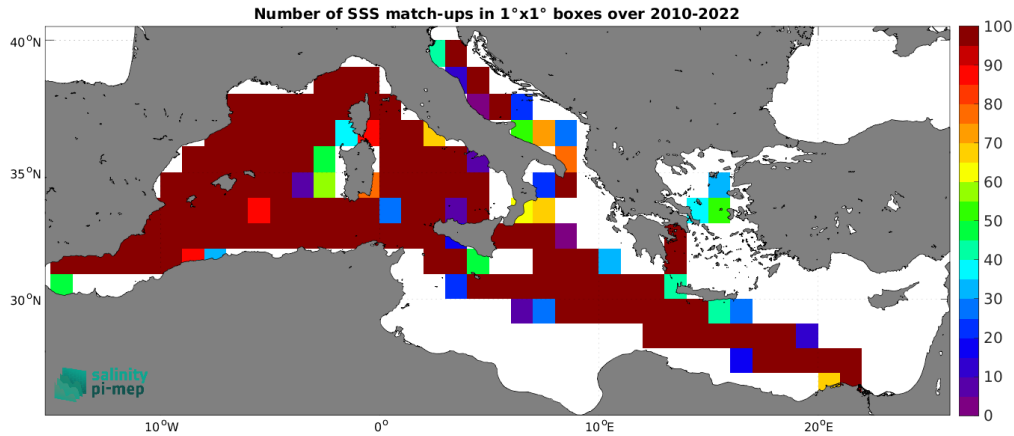
Figure 4: Number of SSS match-ups between TSG (LEGOS-DM) SSS and the SMOS SSS L3 v8 - 9 Days (CATDS-CEC-LOCEAN) SSS product for the Mediterranean Sea Pi-MEP region over 1^\circ \times 1^\circ boxes and for the full satellite product period.
