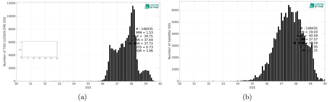
Figure 2: Histograms of SSS from TSG (LEGOS-DM) (a) and SMOS SSS L3 v8 - 9 Days (CATDS-CEC-LOCEAN) (b) considering all match-up pairs per bins of 0.1 over the Mediterranean Sea Pi-MEP region and for the full satellite product period.
