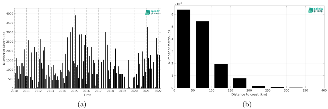
Figure 1: Number of match-ups between TSG (LEGOS-DM) and SMOS SSS L3 v8 - 9 Days (CATDS-CEC-LOCEAN) SSS as a function of time (a) and as function of the distance to coast (b) over the Mediterranean Sea Pi-MEP region and for the full satellite product period.
