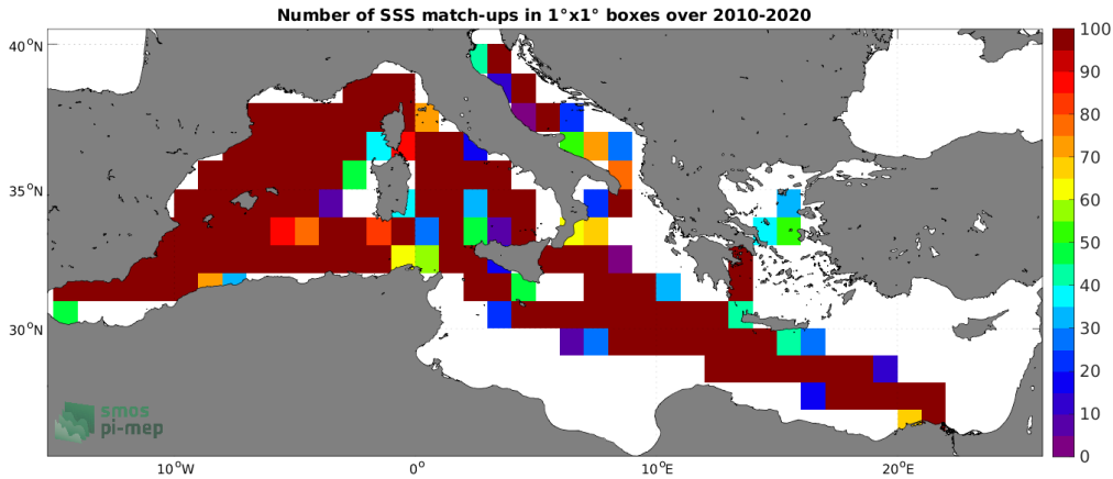
Figure 4: Number of SSS match-ups between TSG (LEGOS-DM) SSS and the SMOS SSS L3 v8 - 9 Days (CATDS-CECOS-LOCEAN) SSS product for the Mediterranean Sea Pi-MEP region over 1^\circ \times 1^\circ boxes and for the full satellite product period.
