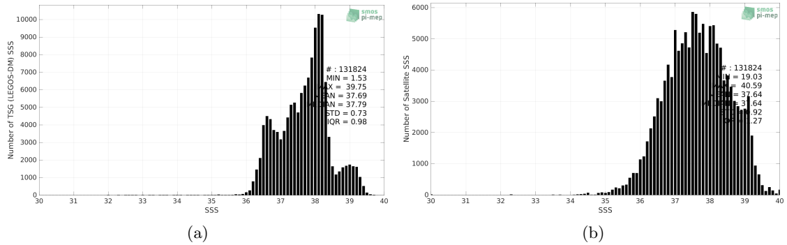
Figure 2: Histograms of SSS from TSG (LEGOS-DM) (a) and SMOS SSS L3 v8 - 9 Days (CATDS-CECOS-LOCEAN) (b) considering all match-up pairs per bins of 0.1 over the Mediterranean Sea Pi-MEP region and for the full satellite product period.
