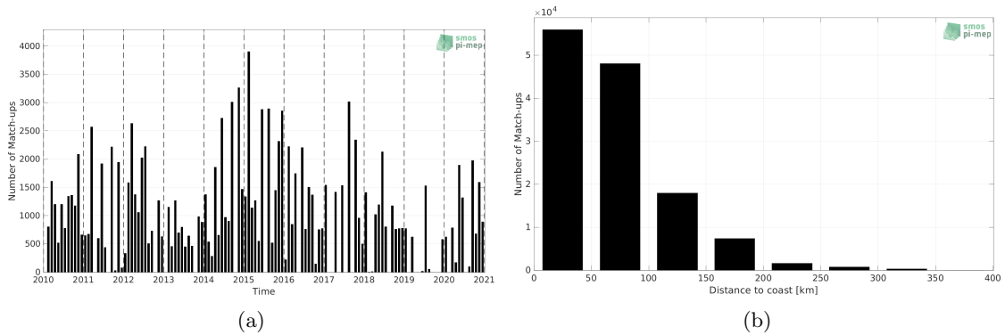
Figure 1: Number of match-ups between TSG (LEGOS-DM) and SMOS SSS L3 v8 - 9 Days (CATDS-CECOS-LOCEAN) SSS as a function of time (a) and as function of the distance to coast (b) over the Mediterranean Sea Pi-MEP region and for the full satellite product period.
