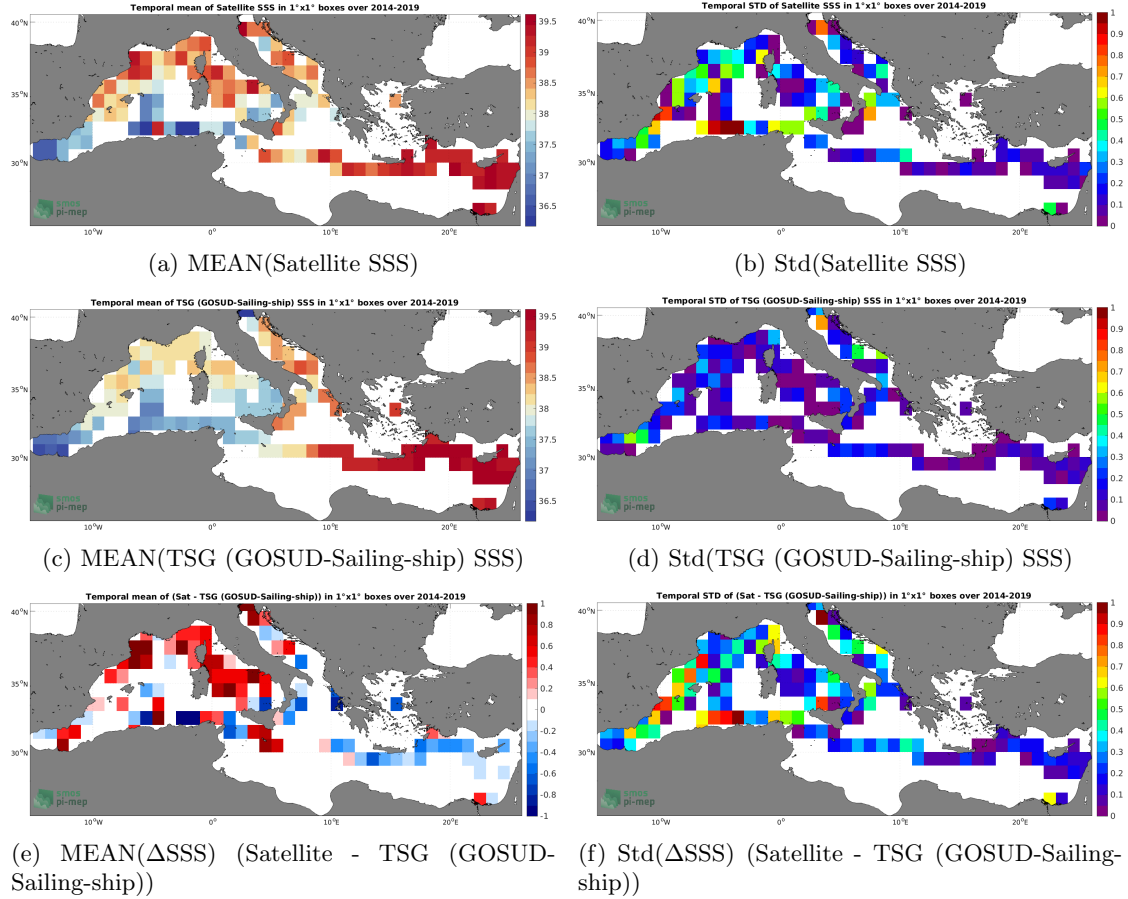
Figure 6: Temporal mean (left) and Std (right) of SSS from SMOS SSS L3 v8 - 9 Days (CATDS-CECOS-LOCEAN) (top), TSG (GOSUD-Sailing-ship) (middle), and of \Delta\text{SSS} (Satellite - TSG (GOSUD-Sailing-ship)). Only match-up pairs are used to generate these maps.
