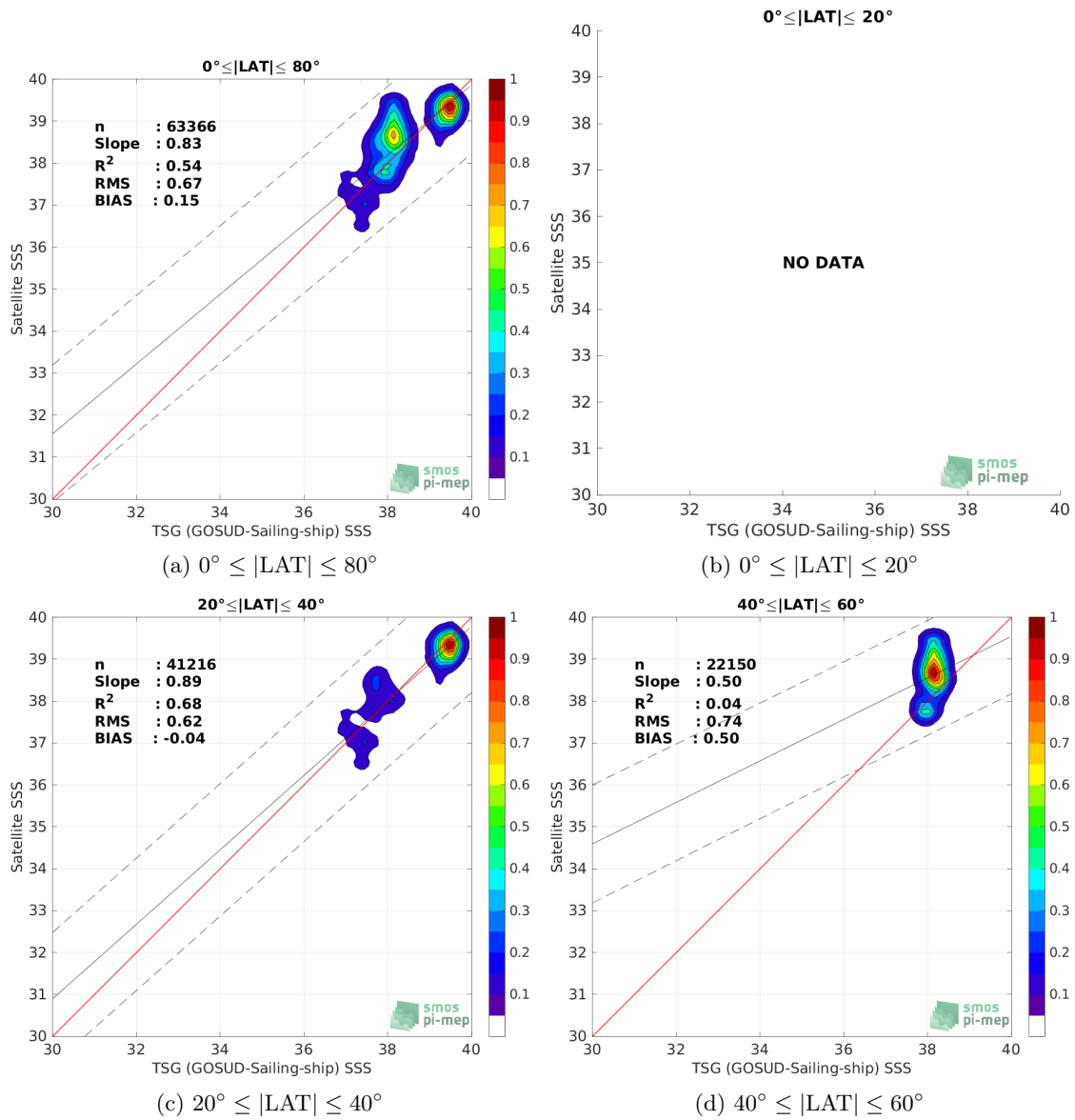
Figure 9: Contour maps of the concentration of SMOS SSS L3 v8 - 9 Days (CATDS-CECOS-LOCEAN) SSS (y-axis) versus TSG (GOSUD-Sailing-ship) SSS (x-axis) at match-up pairs for different latitude bands. For each plot, the red line shows x=y . The black thin and dashed lines indicate a linear fit through the data cloud and the \pm 95\% confidence levels, respectively. The number match-up pairs n , the slope and R^2 coefficient of the linear fit, the root mean square (RMS) and the mean bias between satellite and in situ data are indicated for each latitude band in each plots.
