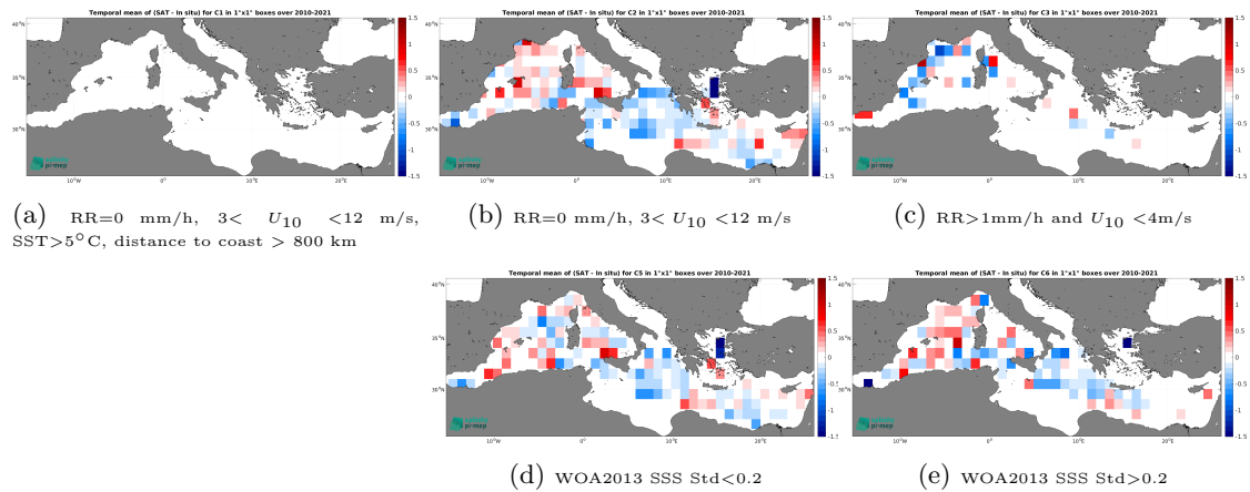
Figure 12: Temporal mean gridded over spatial boxes of size 1^{\circ}\times 1^{\circ} of \Delta SSS (SMOS SSS L3 v8 - 9 Days (CATDS-CEC-LOCEAN) - TSG (GOSUD-Research-vessel)) for 5 different subdatasets corresponding to:RR=0 mm/h, 3 < U_{10} < 12 m/s, SST >5^{\circ}\text{C} , distance to coast > 800 km (a), RR=0 mm/h, 3 < U_{10} < 12 m/s (b), RR >1 mm/h and U_{10} < 4 m/s (c), WOA2013 SSS Std <0.2 (d), WOA2013 SSS Std >0.2 (e).
