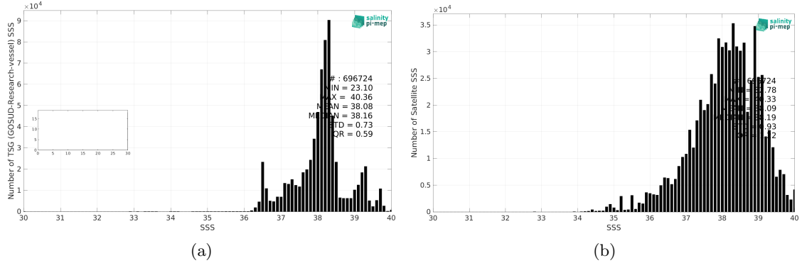
Figure 2: Histograms of SSS from TSG (GOSUD-Research-vessel) (a) and SMOS SSS L3 v8 - 9 Days (CATDS-CEC-LOCEAN) (b) considering all match-up pairs per bins of 0.1 over the Mediterranean Sea Pi-MEP region and for the full satellite product period.
