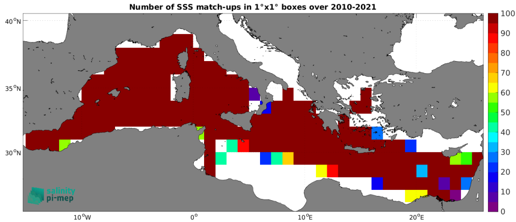
Figure 4: Number of SSS match-ups between TSG (GOSUD-Research-vessel) SSS and the SMOS SSS L3 v8 - 9 Days (CATDS-CEC-LOCEAN) SSS product for the Mediterranean Sea Pi-MEP region over 1^\circ \times 1^\circ boxes and for the full satellite product period.
