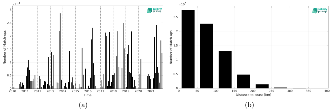
Figure 1: Number of match-ups between TSG (GOSUD-Research-vessel) and SMOS SSS L3 v8 - 9 Days (CATDS-CEC-LOCEAN) SSS as a function of time (a) and as function of the distance to coast (b) over the Mediterranean Sea Pi-MEP region and for the full satellite product period.
