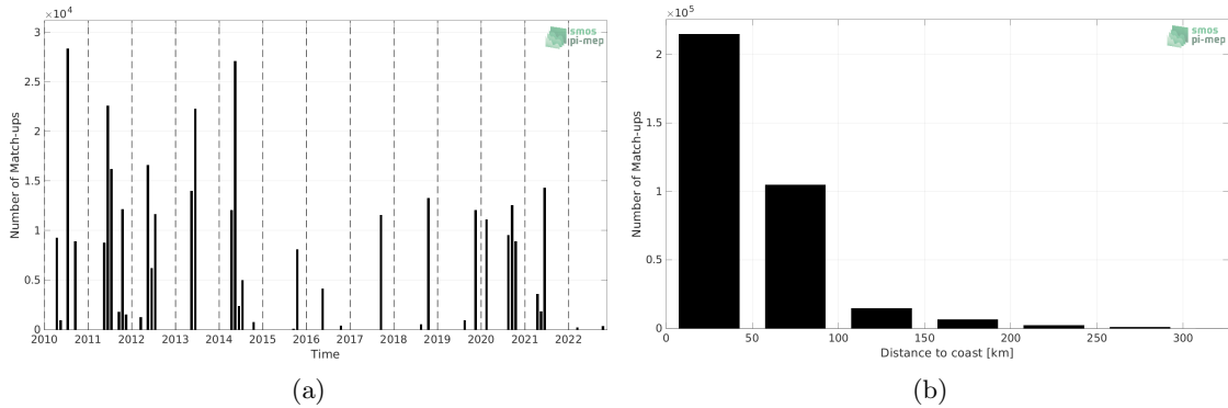
Figure 1: Number of match-ups between TSG (CSIC-UTM) and SMOS SSS L3 v8 - 9 Days (CATDS-CECOS-LOCEAN) SSS as a function of time (a) and as function of the distance to coast (b) over the Mediterranean Sea Pi-MEP region and for the full satellite product period.
