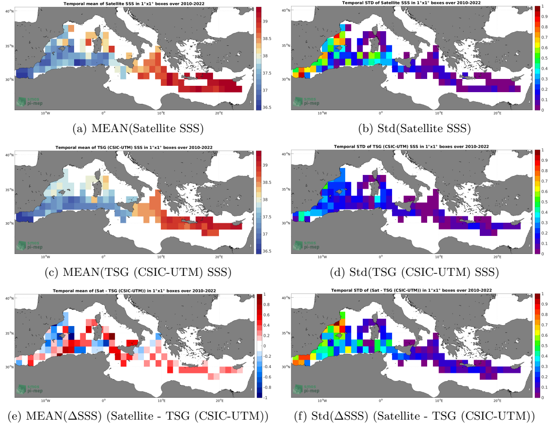
Figure 6: Temporal mean (left) and Std (right) of SSS from SMOS SSS L3 v8 - 9 Days (CATDS-CECOS-LOCEAN) (top), TSG (CSIC-UTM) (middle), and of \Delta\text{SSS} (Satellite - TSG (CSIC-UTM)). Only match-up pairs are used to generate these maps.
