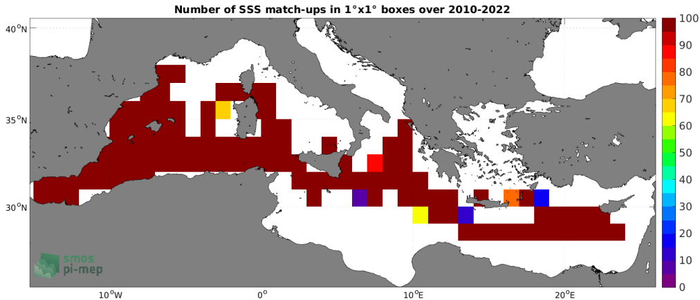
Figure 4: Number of SSS match-ups between TSG (CSIC-UTM) SSS and the SMOS SSS L3 v8 - 9 Days (CATDS-CECOS-LOCEAN) SSS product for the Mediterranean Sea Pi-MEP region over 1^\circ \times 1^\circ boxes and for the full satellite product period.
