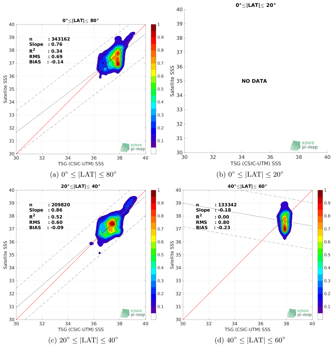
Figure 9: Contour maps of the concentration of SMOS SSS L3 v8 - 9 Days (CATDS-CECOS-LOCEAN) SSS (y-axis) versus TSG (CSIC-UTM) SSS (x-axis) at match-up pairs for different latitude bands. For each plot, the red line shows x=y . The black thin and dashed lines indicate a linear fit through the data cloud and the \pm 95\% confidence levels, respectively. The number match-up pairs n , the slope and R^2 coefficient of the linear fit, the root mean square (RMS) and the mean bias between satellite and in situ data are indicated for each latitude band in each plots.
