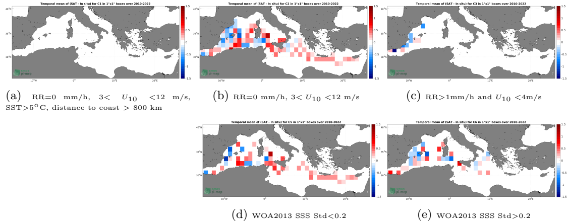
Figure 12: Temporal mean gridded over spatial boxes of size 1^{\circ}\times 1^{\circ} of \Delta\text{SSS} (SMOS SSS L3 v8 - 9 Days (CATDS-CECOS-LOCEAN) - TSG (CSIC-UTM)) for 5 different subdatasets corresponding to:RR=0 mm/h, 3 < U_{10} < 12 m/s, SST >5^{\circ}\text{C} , distance to coast > 800 km (a), RR=0 mm/h, 3 < U_{10} < 12 m/s (b), RR >1 mm/h and U_{10} < 4 m/s (c), WOA2013 SSS Std <0.2 (d), WOA2013 SSS Std >0.2 (e).
