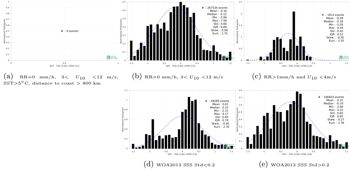
Figure 13: Normalized histogram of \Delta SSS (SMOS SSS L3 v8 - 9 Days (CATDS-CECOS-LOCEAN) - TSG (CSIC-UTM)) for 5 different subdatasets corresponding to: RR=0 mm/h, 3 < U_{10} < 12 m/s, SST > 5°C, distance to coast > 800 km (a), RR=0 mm/h, 3 < U_{10} < 12 m/s (b), RR > 1mm/h and U_{10} < 4 m/s (c), WOA2013 SSS Std < 0.2 (d), WOA2013 SSS Std > 0.2 (e).
