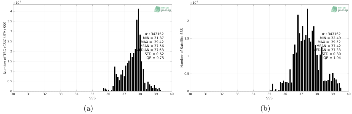
Figure 2: Histograms of SSS from TSG (CSIC-UTM) (a) and SMOS SSS L3 v8 - 9 Days (CATDS-CECOS-LOCEAN) (b) considering all match-up pairs per bins of 0.1 over the Mediterranean Sea Pi-MEP region and for the full satellite product period.
