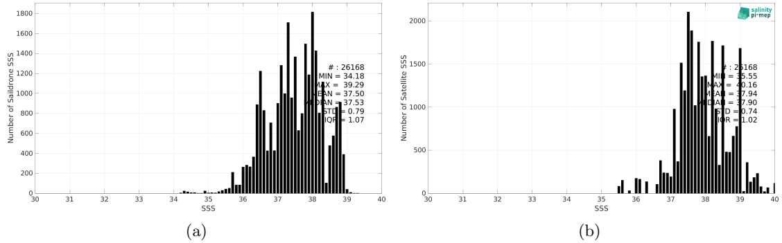
Figure 2: Histograms of SSS from Sairdrone (a) and SMOS SSS L3 v8 - 9 Days (CATDS-CEC-LOCEAN) (b) considering all match-up pairs per bins of 0.1 over the Mediterranean Sea Pi-MEP region and for the full satellite product period.
