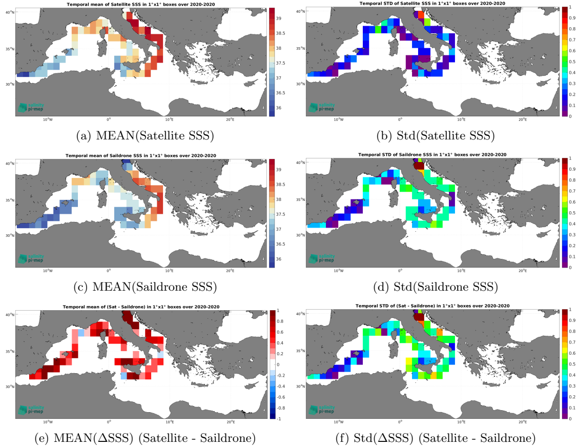
Figure 6: Temporal mean (left) and Std (right) of SSS from SMOS SSS L3 v8 - 9 Days (CATDS-CEC-LOCEAN) (top), Sairdrone (middle), and of \Delta SSS (Satellite - Sairdrone). Only match-up pairs are used to generate these maps.
