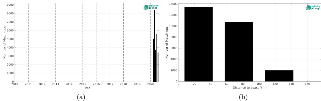
Figure 1: Number of match-ups between Saildrone and SMOS SSS L3 v8 - 9 Days (CATDS-CEC-LOCEAN) SSS as a function of time (a) and as function of the distance to coast (b) over the Mediterranean Sea Pi-MEP region and for the full satellite product period.
