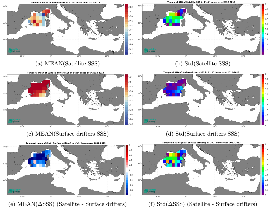
Figure 5: Temporal mean (left) and Std (right) of SSS from SMOS SSS L3 v8 - 9 Days (CATDS-CEC-LOCEAN) (top), Surface drifters (middle), and of \Delta SSS (Satellite - Surface drifters). Only match-up pairs are used to generate these maps.
