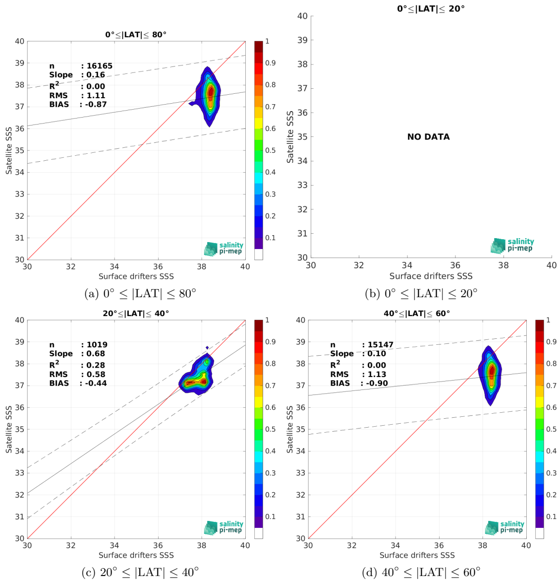
Figure 8: Contour maps of the concentration of SMOS SSS L3 v8 - 9 Days (CATDS-CEC-LOCEAN) SSS (y-axis) versus Surface drifters SSS (x-axis) at match-up pairs for different latitude bands. For each plot, the red line shows x=y . The black thin and dashed lines indicate a linear fit through the data cloud and the \pm 95\% confidence levels, respectively. The number match-up pairs n , the slope and R^2 coefficient of the linear fit, the root mean square (RMS) and the mean bias between satellite and in situ data are indicated for each latitude band in each plots.
