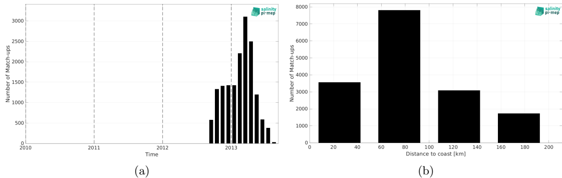
Figure 1: Number of match-ups between Surface drifters and SMOS SSS L3 v8 - 9 Days (CATDS-CEC-LOCEAN) SSS as a function of time (a) and as function of the distance to coast (b) over the Mediterranean Sea Pi-MEP region and for the full satellite product period.
