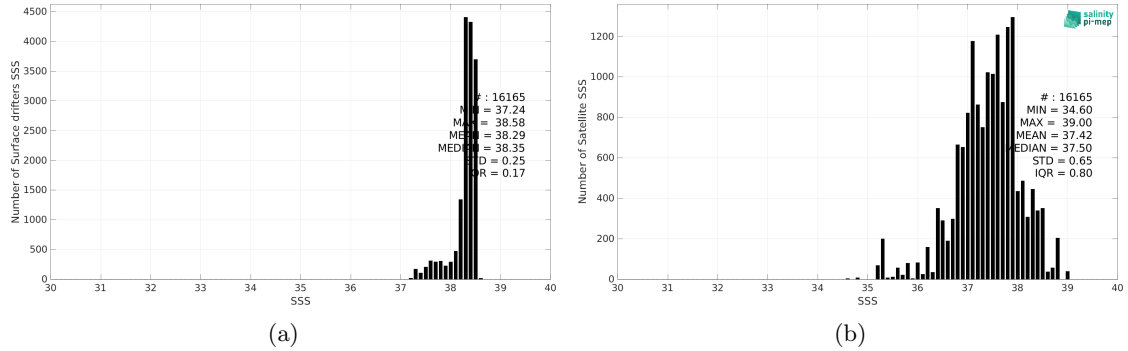
Figure 2: Histograms of SSS from Surface drifters (a) and SMOS SSS L3 v8 - 9 Days (CATDS-CEC-LOCEAN) (b) considering all match-up pairs per bins of 0.1 over the Mediterranean Sea Pi-MEP region and for the full satellite product period.
