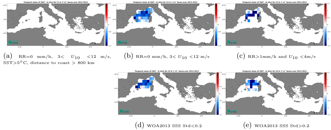
Figure 11: Temporal mean gridded over spatial boxes of size 1^{\circ}\times 1^{\circ} of \Delta\text{SSS} (SMOS SSS L3 v8 - 9 Days (CATDS-CEC-LOCEAN) - Surface drifters) for 5 different subdatasets corresponding to:RR=0 mm/h, 3 < U_{10} < 12 m/s, SST >5^{\circ}\text{C} , distance to coast > 800 km (a), RR=0 mm/h, 3 < U_{10} < 12 m/s (b), RR >1 mm/h and U_{10} < 4 m/s (c), WOA2013 SSS Std <0.2 (d), WOA2013 SSS Std >0.2 (e).
