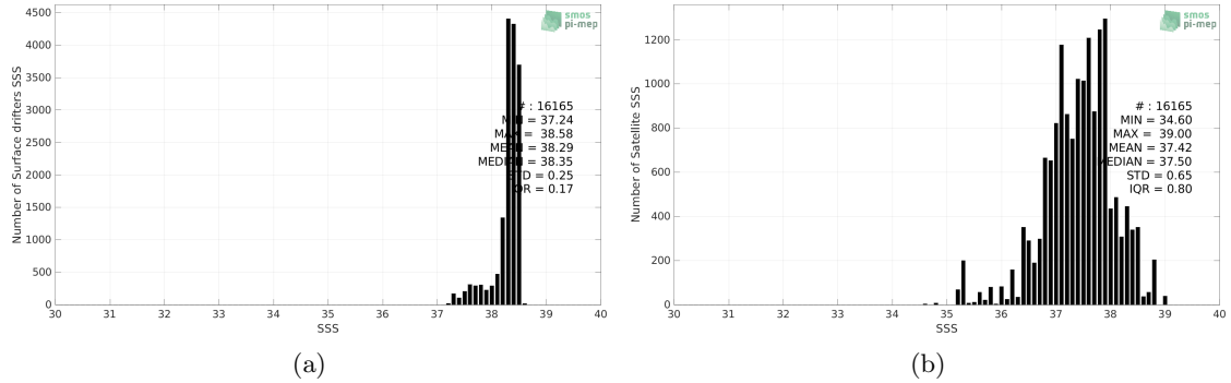
Figure 2: Histograms of SSS from Surface drifters (a) and SMOS SSS L3 v8 - 9 Days (CATDS-CECOS-LOCEAN) (b) considering all match-up pairs per bins of 0.1 over the Mediterranean Sea Pi-MEP region and for the full satellite product period.
