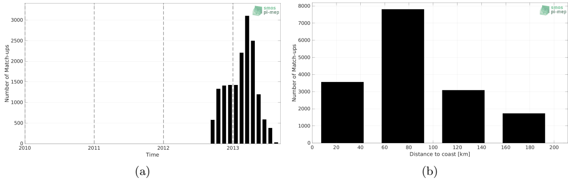
Figure 1: Number of match-ups between Surface drifters and SMOS SSS L3 v8 - 9 Days (CATDS-CECOS-LOCEAN) SSS as a function of time (a) and as function of the distance to coast (b) over the Mediterranean Sea Pi-MEP region and for the full satellite product period.
