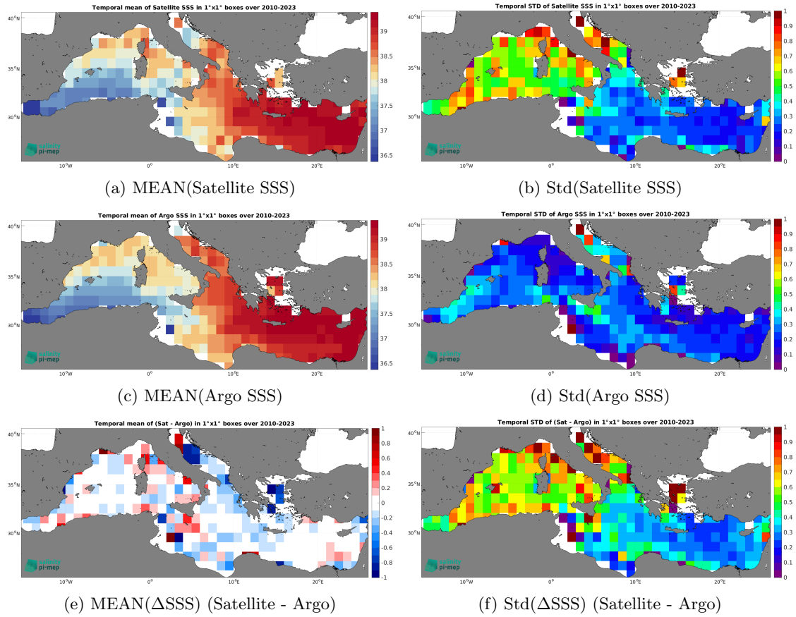
Figure 6: Temporal mean (left) and Std (right) of SSS from SMOS SSS L3 v8 - 9 Days (CATDS-CEC-LOCEAN) (top), Argo (middle), and of \Delta SSS (Satellite - Argo). Only match-up pairs are used to generate these maps.
