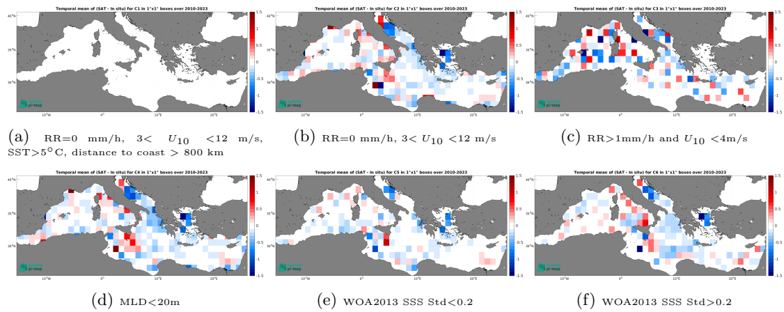
Figure 12: Temporal mean gridded over spatial boxes of size 1^\circ \times 1^\circ of \Delta SSS (SMOS SSS L3 v8 - 9 Days (CATDS-CEC-LOCEAN) - Argo) for 6 different subdatasets corresponding to:RR=0 mm/h, 3 < U_{10} < 12 m/s, SST > 5^\circ C , distance to coast > 800 km (a), RR=0 mm/h, 3 < U_{10} < 12 m/s (b), RR >1 mm/h and U_{10} < 4 m/s (c),MLD <20 m (d),WOA2013 SSS Std <0.2 (e),WOA2013 SSS Std >0.2 (f).
