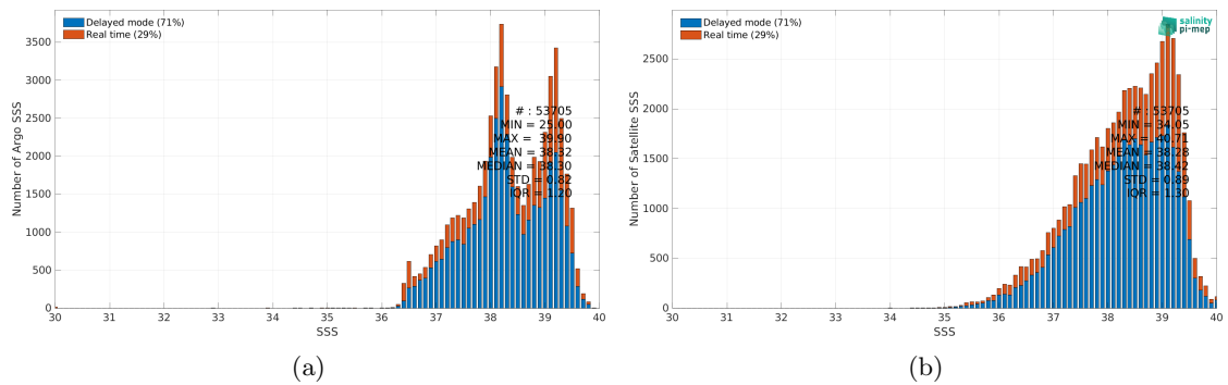
Figure 2: Histograms of SSS from Argo (a) and SMOS SSS L3 v8 - 9 Days (CATDS-CEC-LOCEAN) (b) considering all match-up pairs per bins of 0.1 over the Mediterranean Sea Pi-MEP region and for the full satellite product period.
