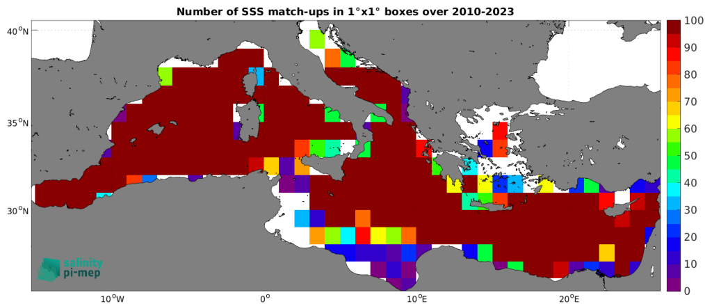
Figure 4: Number of SSS match-ups between Argo SSS and the SMOS SSS L3 v8 - 9 Days (CATDS-CEC-LOCEAN) SSS product for the Mediterranean Sea Pi-MEP region over 1^\circ \times 1^\circ boxes and for the full satellite product period.
