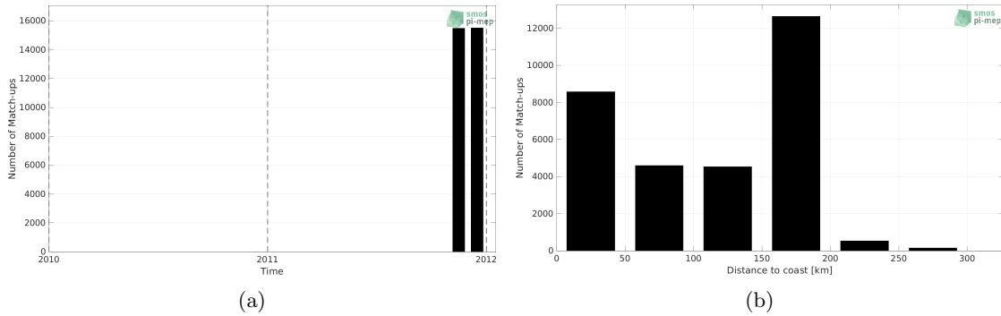
Figure 1: Number of match-ups between TSG (SAMOS) and SMOS SSS L3 v8 - 18 Days (CATDS-CECOS-LOCEAN) SSS as a function of time (a) and as function of the distance to coast (b) over the Mediterranean Sea Pi-MEP region and for the full satellite product period.
