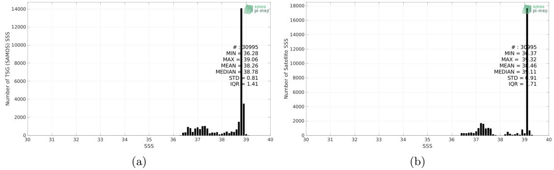
Figure 2: Histograms of SSS from TSG (SAMOS) (a) and SMOS SSS L3 v8 - 18 Days (CATDS-CECOS-LOCEAN) (b) considering all match-up pairs per bins of 0.1 over the Mediterranean Sea Pi-MEP region and for the full satellite product period.
