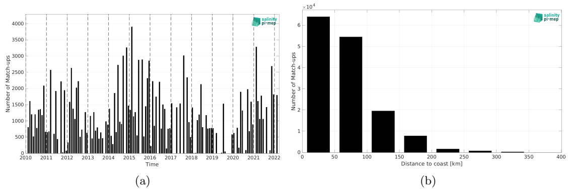
Figure 1: Number of match-ups between TSG (LEGOS-DM) and SMOS SSS L3 v8 - 18 Days (CATDS-CEC-LOCEAN) SSS as a function of time (a) and as function of the distance to coast (b) over the Mediterranean Sea Pi-MEP region and for the full satellite product period.
