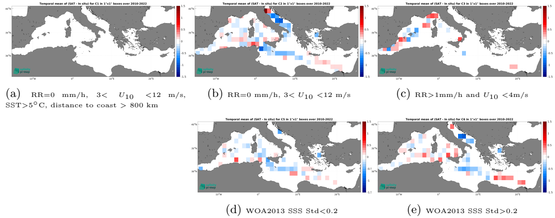
Figure 12: Temporal mean gridded over spatial boxes of size 1^{\circ}\times 1^{\circ} of \Delta\text{SSS} (SMOS SSS L3 v8 - 18 Days (CATDS-CEC-LOCEAN) - TSG (LEGOS-DM)) for 5 different subdatasets corresponding to:RR=0 mm/h, 3 < U_{10} < 12 m/s, SST >5^{\circ}\text{C} , distance to coast > 800 km (a), RR=0 mm/h, 3 < U_{10} < 12 m/s (b), RR >1 mm/h and U_{10} < 4 m/s (c), WOA2013 SSS Std <0.2 (d), WOA2013 SSS Std >0.2 (e).
