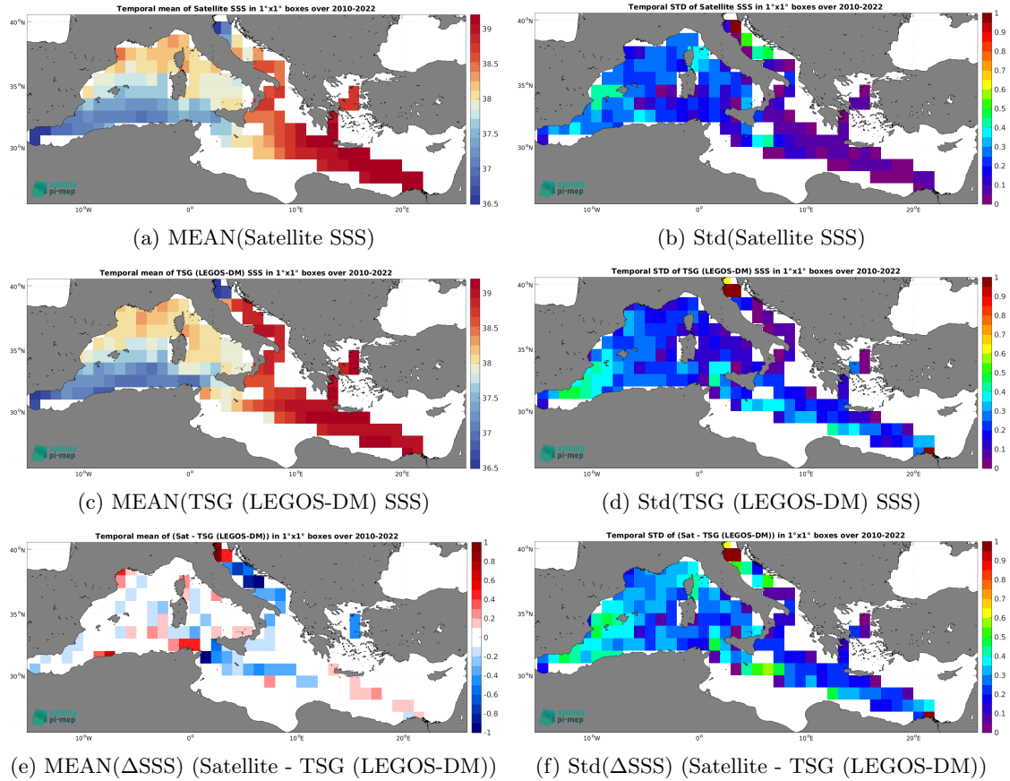
Figure 6: Temporal mean (left) and Std (right) of SSS from SMOS SSS L3 v8 - 18 Days (CATDS-CEC-LOCEAN) (top), TSG (LEGOS-DM) (middle), and of \Delta\text{SSS} (Satellite - TSG (LEGOS-DM)). Only match-up pairs are used to generate these maps.
