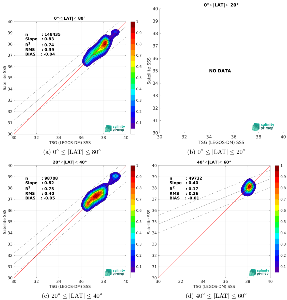
Figure 9: Contour maps of the concentration of SMOS SSS L3 v8 - 18 Days (CATDS-CEC-LOCEAN) SSS (y-axis) versus TSG (LEGOS-DM) SSS (x-axis) at match-up pairs for different latitude bands. For each plot, the red line shows x=y . The black thin and dashed lines indicate a linear fit through the data cloud and the \pm 95\% confidence levels, respectively. The number match-up pairs n , the slope and R^2 coefficient of the linear fit, the root mean square (RMS) and the mean bias between satellite and in situ data are indicated for each latitude band in each plots.
