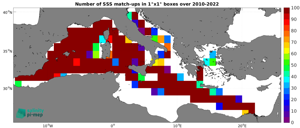
Figure 4: Number of SSS match-ups between TSG (LEGOS-DM) SSS and the SMOS SSS L3 v8 - 18 Days (CATDS-CEC-LOCEAN) SSS product for the Mediterranean Sea Pi-MEP region over 1^\circ \times 1^\circ boxes and for the full satellite product period.
