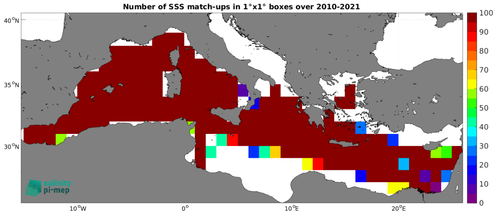
Figure 4: Number of SSS match-ups between TSG (GOSUD-Research-vessel) SSS and the SMOS SSS L3 v8 - 18 Days (CATDS-CEC-LOCEAN) SSS product for the Mediterranean Sea Pi-MEP region over 1^\circ \times 1^\circ boxes and for the full satellite product period.
