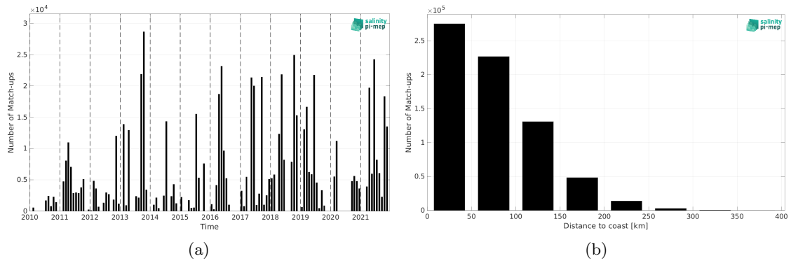
Figure 1: Number of match-ups between TSG (GOSUD-Research-vessel) and SMOS SSS L3 v8 - 18 Days (CATDS-CEC-LOCEAN) SSS as a function of time (a) and as function of the distance to coast (b) over the Mediterranean Sea Pi-MEP region and for the full satellite product period.
