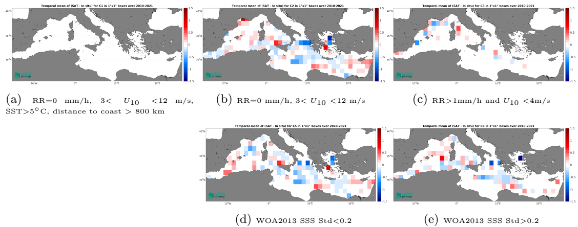
Figure 12: Temporal mean gridded over spatial boxes of size 1^{\circ}\times 1^{\circ} of \Delta SSS (SMOS SSS L3 v8 - 18 Days (CATDS-CEC-LOCEAN) - TSG (GOSUD-Research-vessel)) for 5 different subdatasets corresponding to:RR=0 mm/h, 3 < U_{10} < 12 m/s, SST >5^{\circ}\text{C} , distance to coast > 800 km (a), RR=0 mm/h, 3 < U_{10} < 12 m/s (b), RR >1 mm/h and U_{10} < 4 m/s (c), WOA2013 SSS Std <0.2 (d), WOA2013 SSS Std >0.2 (e).
