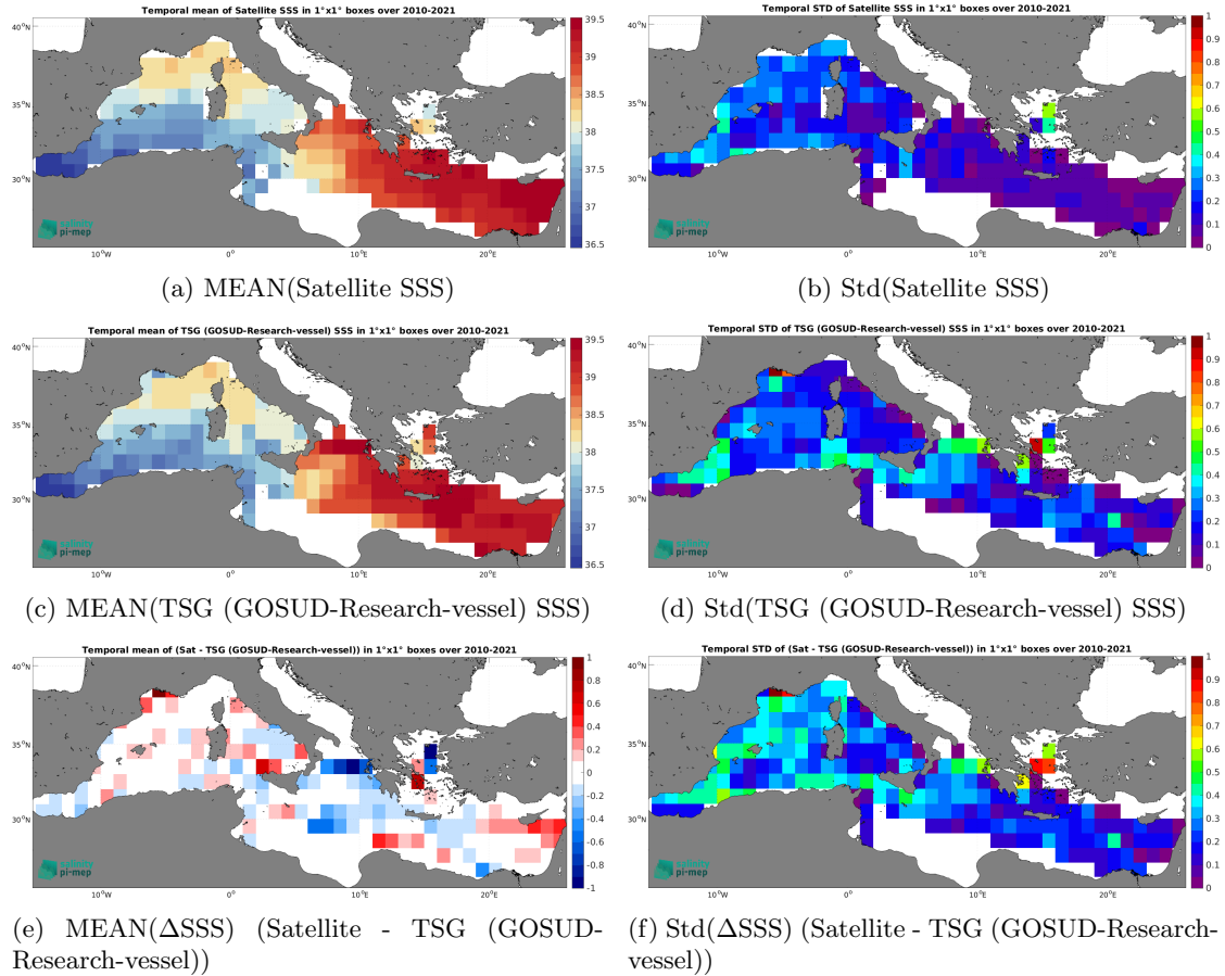
Figure 6: Temporal mean (left) and Std (right) of SSS from SMOS SSS L3 v8 - 18 Days (CATDS-CEC-LOCEAN) (top), TSG (GOSUD-Research-vessel) (middle), and of \Delta\text{SSS} (Satellite - TSG (GOSUD-Research-vessel)). Only match-up pairs are used to generate these maps.
