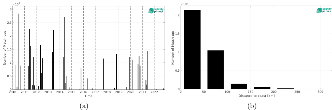
Figure 1: Number of match-ups between TSG (CSIC-UTM) and SMOS SSS L3 v8 - 18 Days (CATDS-CEC-LOCEAN) SSS as a function of time (a) and as function of the distance to coast (b) over the Mediterranean Sea Pi-MEP region and for the full satellite product period.
