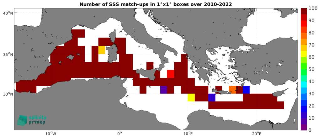
Figure 4: Number of SSS match-ups between TSG (CSIC-UTM) SSS and the SMOS SSS L3 v8 - 18 Days (CATDS-CEC-LOCEAN) SSS product for the Mediterranean Sea Pi-MEP region over 1^\circ \times 1^\circ boxes and for the full satellite product period.
