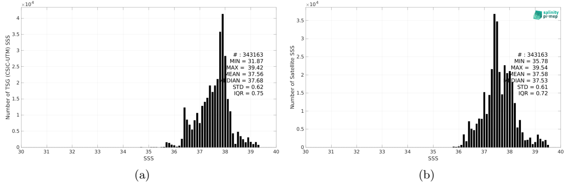
Figure 2: Histograms of SSS from TSG (CSIC-UTM) (a) and SMOS SSS L3 v8 - 18 Days (CATDS-CEC-LOCEAN) (b) considering all match-up pairs per bins of 0.1 over the Mediterranean Sea Pi-MEP region and for the full satellite product period.
