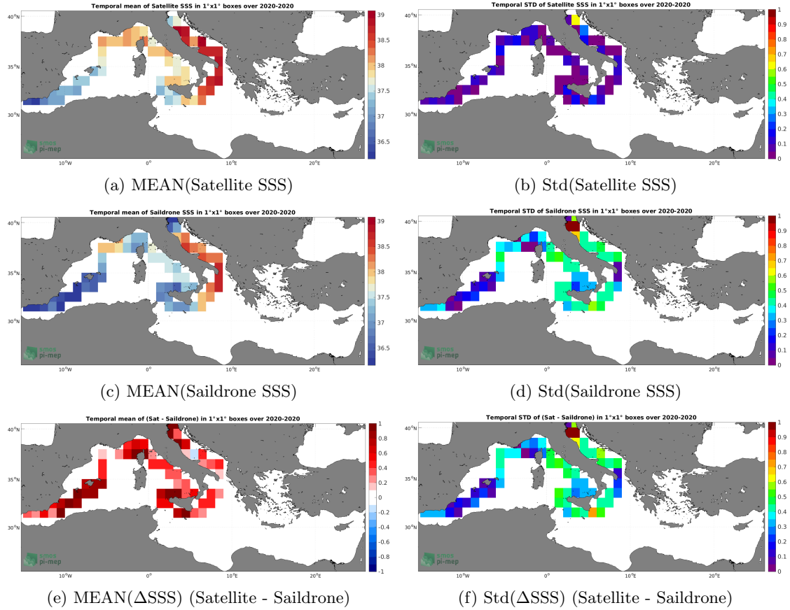
Figure 6: Temporal mean (left) and Std (right) of SSS from SMOS SSS L3 v8 - 18 Days (CATDS-CECOS-LOCEAN) (top), Sairdron (middle), and of \Delta SSS (Satellite - Sairdron). Only match-up pairs are used to generate these maps.
