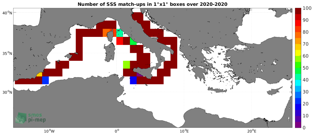
Figure 4: Number of SSS match-ups between Sairdrone SSS and the SMOS SSS L3 v8 - 18 Days (CATDS-CECOS-LOCEAN) SSS product for the Mediterranean Sea Pi-MEP region over 1^\circ \times 1^\circ boxes and for the full satellite product period.
