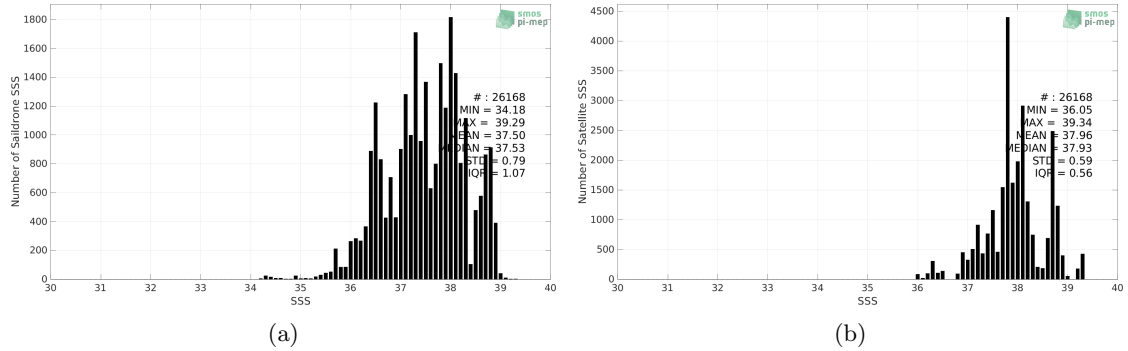
Figure 2: Histograms of SSS from Saildrone (a) and SMOS SSS L3 v8 - 18 Days (CATDS-CECOS-LOCEAN) (b) considering all match-up pairs per bins of 0.1 over the Mediterranean Sea Pi-MEP region and for the full satellite product period.
