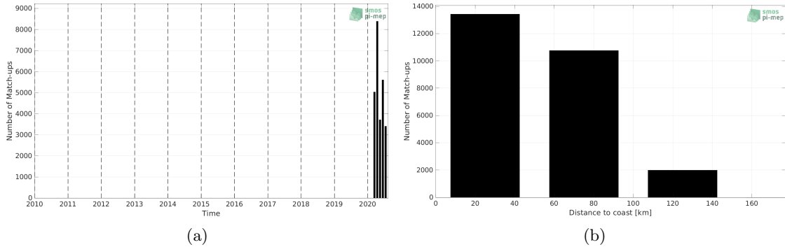
Figure 1: Number of match-ups between Saildrone and SMOS SSS L3 v8 - 18 Days (CATDS-CECOS-LOCEAN) SSS as a function of time (a) and as function of the distance to coast (b) over the Mediterranean Sea Pi-MEP region and for the full satellite product period.
