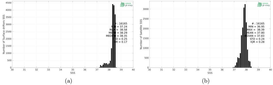
Figure 2: Histograms of SSS from Surface drifters (a) and SMOS SSS L3 v8 - 18 Days (CATDS-CECOS-LOCEAN) (b) considering all match-up pairs per bins of 0.1 over the Mediterranean Sea Pi-MEP region and for the full satellite product period.
