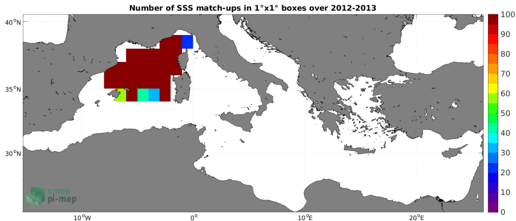
Figure 3: Number of SSS match-ups between Surface drifters SSS and the SMOS SSS L3 v8 - 18 Days (CATDS-CECOS-LOCEAN) SSS product for the Mediterranean Sea Pi-MEP region over 1^\circ \times 1^\circ boxes and for the full satellite product period.
