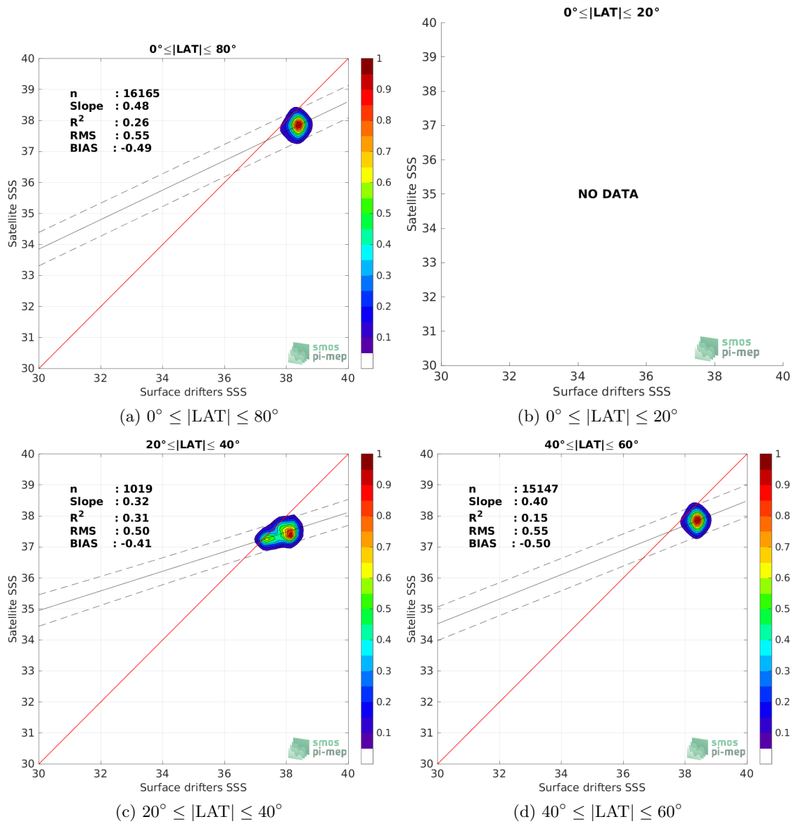
Figure 8: Contour maps of the concentration of SMOS SSS L3 v8 - 18 Days (CATDS-CECOS-LOCEAN) SSS ( y -axis) versus Surface drifters SSS ( x -axis) at match-up pairs for different latitude bands. For each plot, the red line shows x=y . The black thin and dashed lines indicate a linear fit through the data cloud and the \pm 95\% confidence levels, respectively. The number match-up pairs n , the slope and R^2 coefficient of the linear fit, the root mean square (RMS) and the mean bias between satellite and in situ data are indicated for each latitude band in each plots.
