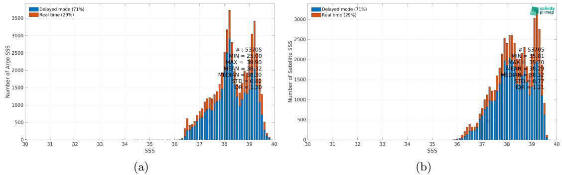
Figure 2: Histograms of SSS from Argo (a) and SMOS SSS L3 v8 - 18 Days (CATDS-CEC-LOCEAN) (b) considering all match-up pairs per bins of 0.1 over the Mediterranean Sea Pi-MEP region and for the full satellite product period.
