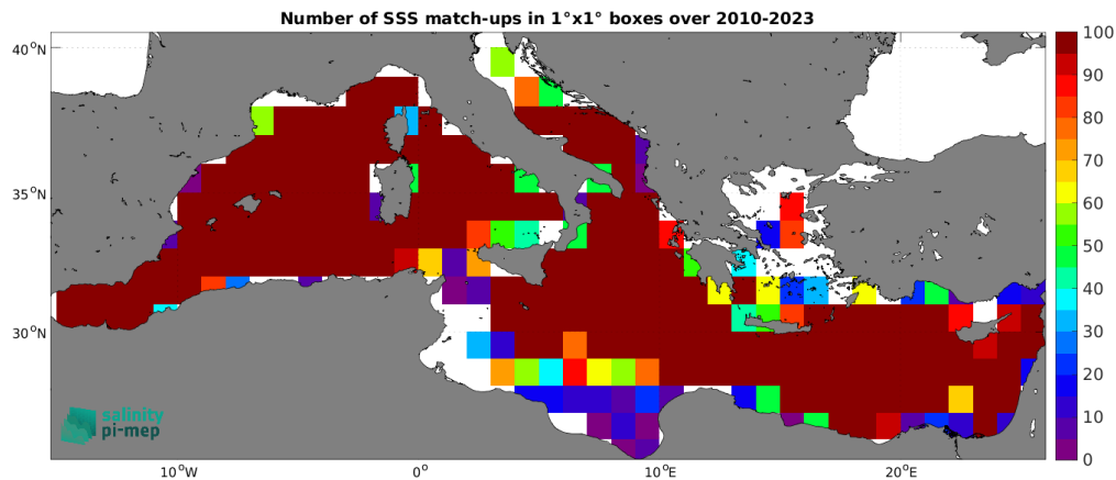
Figure 4: Number of SSS match-ups between Argo SSS and the SMOS SSS L3 v8 - 18 Days (CATDS-CEC-LOCEAN) SSS product for the Mediterranean Sea Pi-MEP region over 1^\circ \times 1^\circ boxes and for the full satellite product period.
