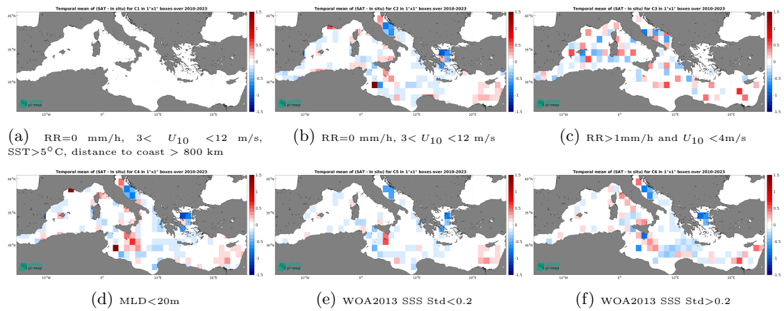
Figure 12: Temporal mean gridded over spatial boxes of size 1^\circ \times 1^\circ of \Delta SSS (SMOS SSS L3 v8 - 18 Days (CATDS-CEC-LOCEAN) - Argo) for 6 different subdatasets corresponding to:RR=0 mm/h, 3 < U_{10} < 12 m/s, SST >5^\circ C, distance to coast > 800 km (a), RR=0 mm/h, 3 < U_{10} < 12 m/s (b), RR >1 mm/h and U_{10} < 4 m/s (c),MLD <20 m (d),WOA2013 SSS Std <0.2 (e),WOA2013 SSS Std >0.2 (f).
