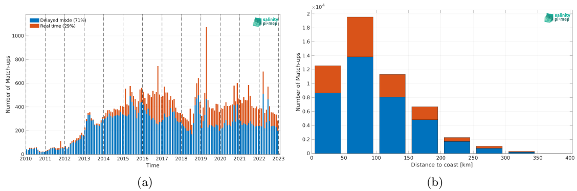
Figure 1: Number of match-ups between Argo and SMOS SSS L3 v8 - 18 Days (CATDS-CEC-LOCEAN) SSS as a function of time (a) and as function of the distance to coast (b) over the Mediterranean Sea Pi-MEP region and for the full satellite product period.
