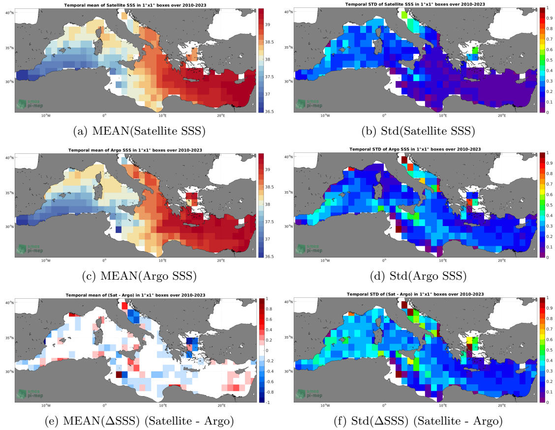
Figure 6: Temporal mean (left) and Std (right) of SSS from SMOS SSS L3 v8 - 18 Days (CATDS-CECOS-LOCEAN) (top), Argo (middle), and of \Delta SSS (Satellite - Argo). Only match-up pairs are used to generate these maps.
