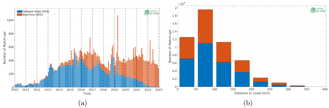
Figure 1: Number of match-ups between Argo and SMOS SSS L3 v8 - 18 Days (CATDS-CECOS-LOCEAN) SSS as a function of time (a) and as function of the distance to coast (b) over the Mediterranean Sea Pi-MEP region and for the full satellite product period.
