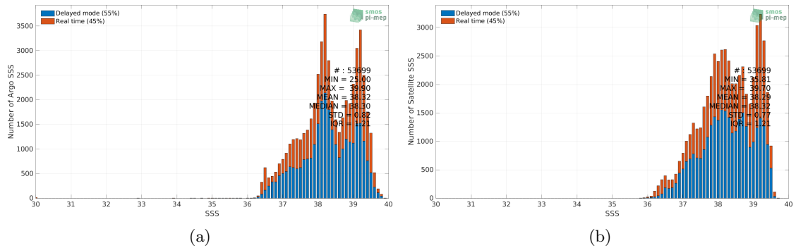
Figure 2: Histograms of SSS from Argo (a) and SMOS SSS L3 v8 - 18 Days (CATDS-CECOS-LOCEAN) (b) considering all match-up pairs per bins of 0.1 over the Mediterranean Sea Pi-MEP region and for the full satellite product period.
