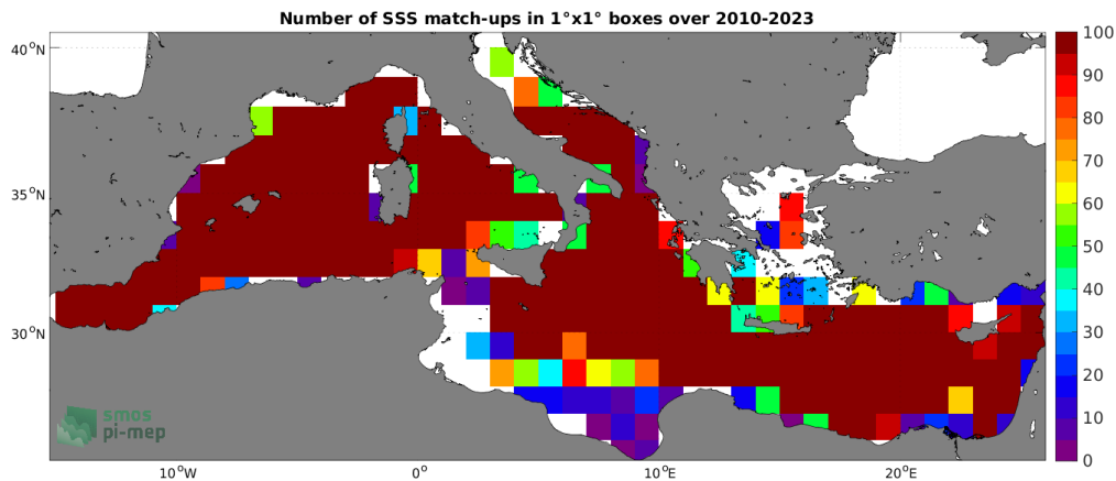
Figure 4: Number of SSS match-ups between Argo SSS and the SMOS SSS L3 v8 - 18 Days (CATDS-CECOS-LOCEAN) SSS product for the Mediterranean Sea Pi-MEP region over 1^\circ \times 1^\circ boxes and for the full satellite product period.
