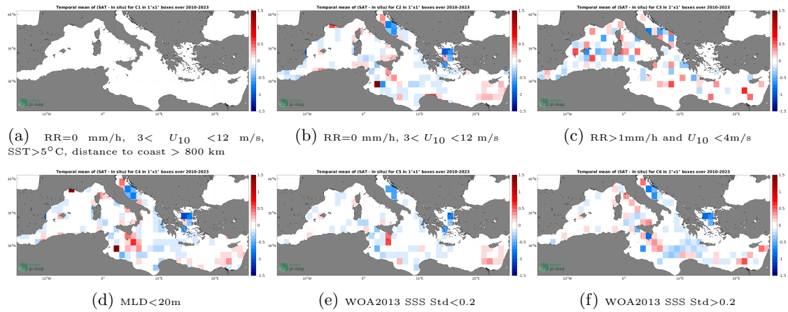
Figure 12: Temporal mean gridded over spatial boxes of size 1^\circ \times 1^\circ of \Delta SSS (SMOS SSS L3 v8 - 18 Days (CATDS-CECOS-LOCEAN) - Argo) for 6 different subdatasets corresponding to:RR=0 mm/h, 3 < U_{10} < 12 m/s, SST >5^\circ C, distance to coast > 800 km (a), RR=0 mm/h, 3 < U_{10} < 12 m/s (b), RR >1 mm/h and U_{10} < 4 m/s (c),MLD <20 m (d),WOA2013 SSS Std <0.2 (e),WOA2013 SSS Std >0.2 (f).
