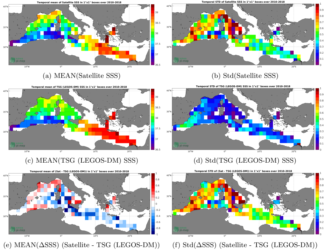
Figure 6: Temporal mean (left) and Std (right) of SSS from SMOS SSS L3 v5 - 9 Days (CATDS-CECOS-LOCEAN) (top), TSG (LEGOS-DM) ( in situ ) dataset (middle), and of \Delta SSS (Satellite - TSG (LEGOS-DM)). Only match-up pairs are used to generate these maps.
