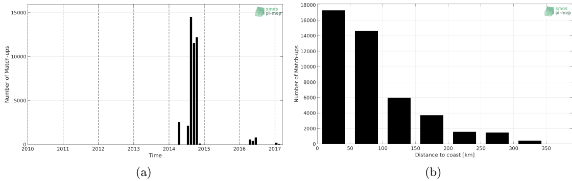
Figure 1: Number of match-ups between TSG (GOSUD-Sailing-ship) and SMOS SSS L3 v5 - 9 Days (CATDS-CECOS-LOCEAN) SSS as a function of time (a) and as function of the distance to coast (b) over the Mediterranean Sea Pi-MEP region and for the full satellite product period.
