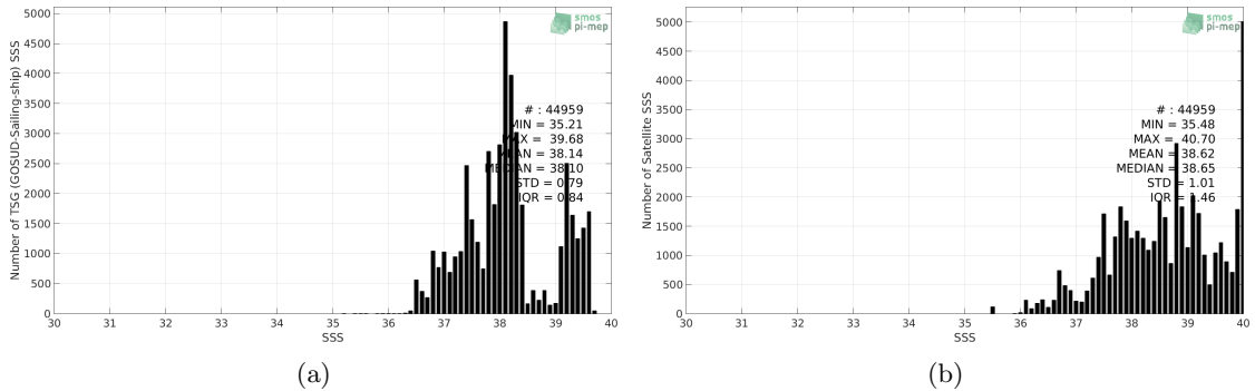
Figure 2: Histograms of SSS from TSG (GOSUD-Sailing-ship) (a) and SMOS SSS L3 v5 - 9 Days (CATDS-CECOS-LOCEAN) (b) considering all match-up pairs per bins of 0.1 over the Mediterranean Sea Pi-MEP region and for the full satellite product period.
