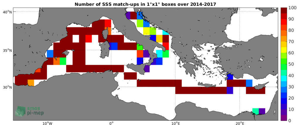
Figure 4: Number of SSS match-ups between TSG (GOSUD-Sailing-ship) SSS and the SMOS SSS L3 v5 - 9 Days (CATDS-CECOS-LOCEAN) SSS product for the Mediterranean Sea Pi-MEP region over 1^\circ \times 1^\circ boxes and for the full satellite product period.
