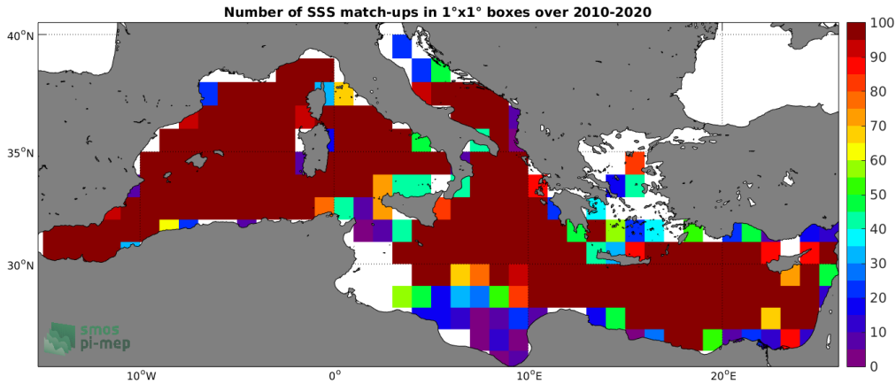
Figure 4: Number of SSS match-ups between Argo SSS and the SMOS SSS L3 v5 - 9 Days (CATDS-CECOS-LOCEAN) SSS product for the Mediterranean Sea Pi-MEP region over 1^\circ \times 1^\circ boxes and for the full satellite product period.
