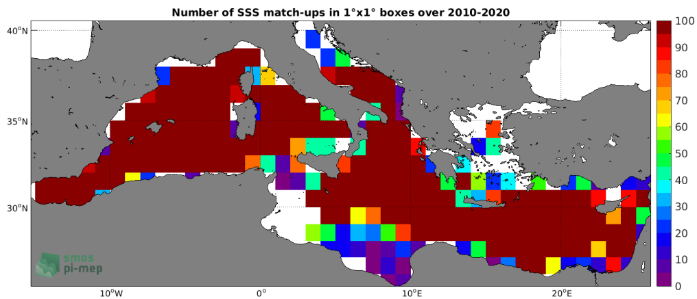
Figure 4: Number of SSS match-ups between Argos SSS and the SMOS SSS L3 v5 - 9 Days (CATDS-CECOS-LOCEAN) SSS product for the Mediterranean Sea Pi-MEP region over 1^\circ \times 1^\circ boxes and for the full satellite product period.
