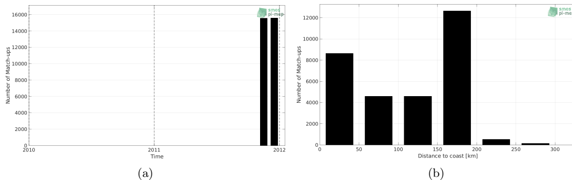
Figure 1: Number of match-ups between TSG (SAMOS) and SMOS SSS L3 v5 - 18 Days (CATDS-CECOS-LOCEAN) SSS as a function of time (a) and as function of the distance to coast (b) over the Mediterranean Sea Pi-MEP region and for the full satellite product period.
