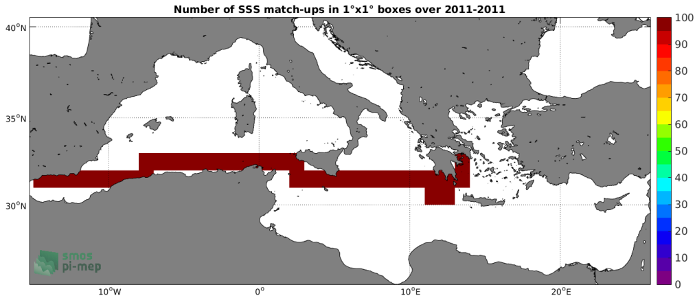
Figure 4: Number of SSS match-ups between TSG (SAMOS) SSS and the SMOS SSS L3 v5 - 18 Days (CATDS-CECOS-LOCEAN) SSS product for the Mediterranean Sea Pi-MEP region over 1^\circ \times 1^\circ boxes and for the full satellite product period.
