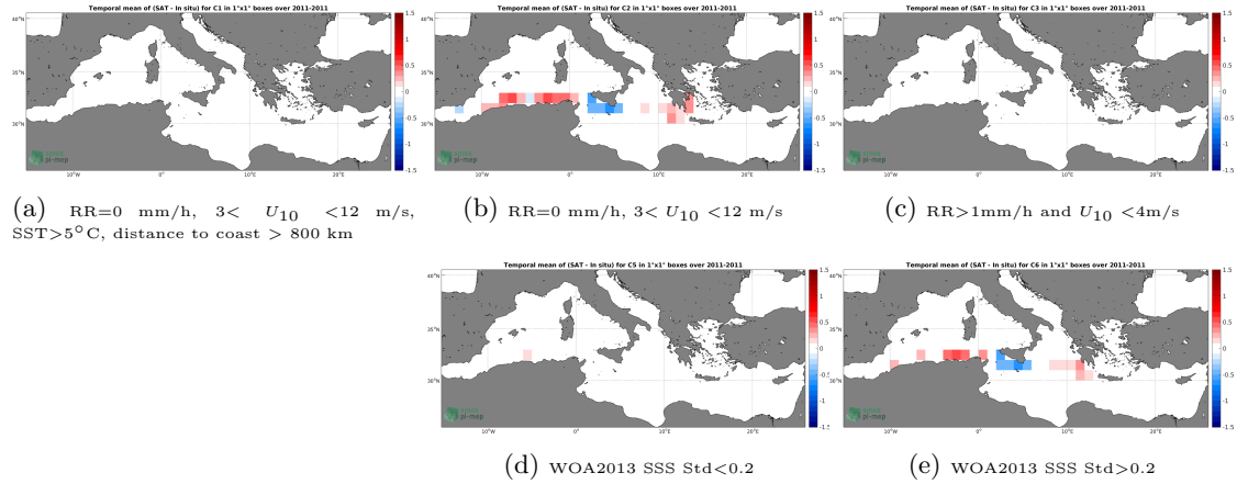
Figure 12: Temporal mean gridded over spatial boxes of size 1^{\circ}\times 1^{\circ} of \Delta\text{SSS} (SMOS SSS L3 v5 - 18 Days (CATDS-CECOS-LOCEAN) - TSG (SAMOS)) for 5 different subdatasets corresponding to:RR=0 mm/h, 3 < U_{10} < 12 m/s, SST >5^{\circ}\text{C} , distance to coast > 800 km (a), RR=0 mm/h, 3 < U_{10} < 12 m/s (b), RR >1 mm/h and U_{10} < 4 m/s (c), WOA2013 SSS Std <0.2 (d), WOA2013 SSS Std >0.2 (e).
