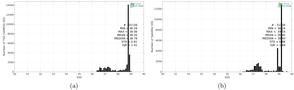
Figure 2: Histograms of SSS from TSG (SAMOS) (a) and SMOS SSS L3 v5 - 18 Days (CATDS-CECOS-LOCEAN) (b) considering all match-up pairs per bins of 0.1 over the Mediterranean Sea Pi-MEP region and for the full satellite product period.
