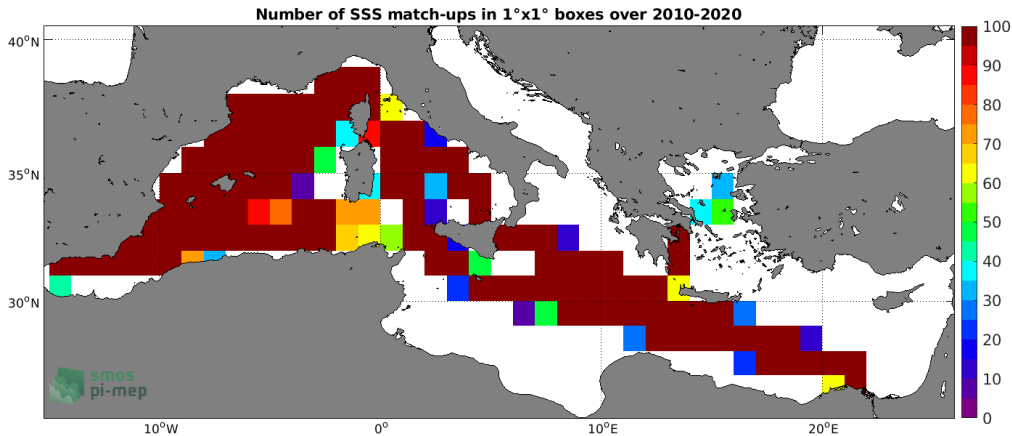
Figure 4: Number of SSS match-ups between TSG (LEGOS-DM) SSS and the SMOS SSS L3 v5 - 18 Days (CATDS-CECOS-LOCEAN) SSS product for the Mediterranean Sea Pi-MEP region over 1°x1° boxes and for the full satellite product period.
