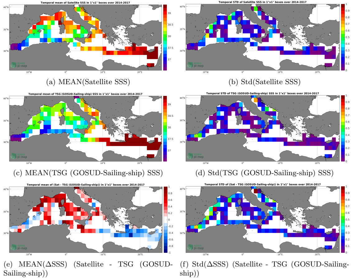
Figure 6: Temporal mean (left) and Std (right) of SSS from SMOS SSS L3 v5 - 18 Days (CATDS-CECOS-LOCEAN) (top), TSG (GOSUD-Sailing-ship) (middle), and of \Delta\text{SSS} (Satellite - TSG (GOSUD-Sailing-ship)). Only match-up pairs are used to generate these maps.
