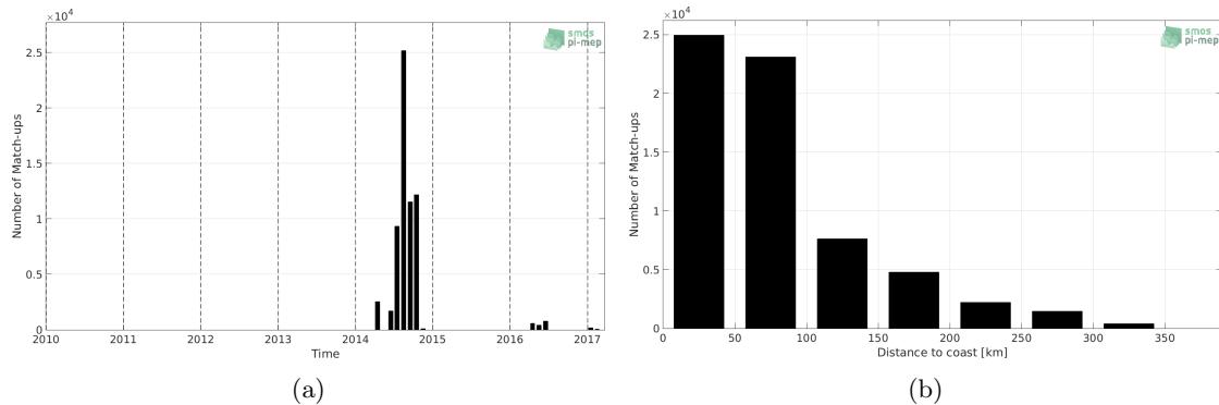
Figure 1: Number of match-ups between TSG (GOSUD-Sailing-ship) and SMOS SSS L3 v5 - 18 Days (CATDS-CECOS-LOCEAN) SSS as a function of time (a) and as function of the distance to coast (b) over the Mediterranean Sea Pi-MEP region and for the full satellite product period.
