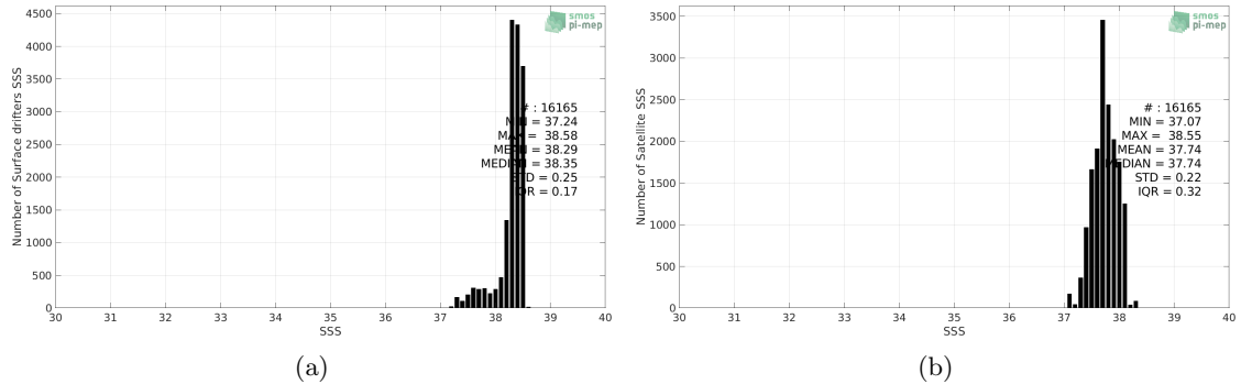
Figure 2: Histograms of SSS from Surface drifters (a) and SMOS SSS L3 v5 - 18 Days (CATDS-CECOS-LOCEAN) (b) considering all match-up pairs per bins of 0.1 over the Mediterranean Sea Pi-MEP region and for the full satellite product period.
