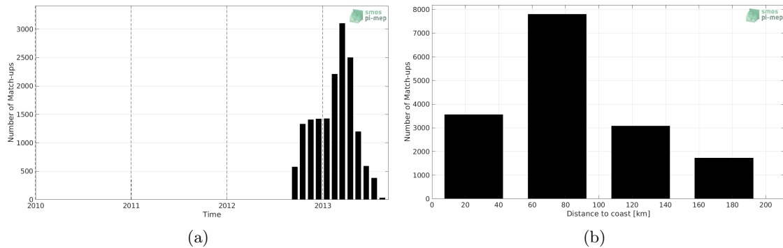
Figure 1: Number of match-ups between Surface drifters and SMOS SSS L3 v5 - 18 Days (CATDS-CECOS-LOCEAN) SSS as a function of time (a) and as function of the distance to coast (b) over the Mediterranean Sea Pi-MEP region and for the full satellite product period.
