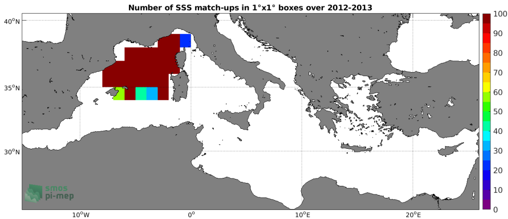
Figure 3: Number of SSS match-ups between Surface drifters SSS and the SMOS SSS L3 v5 - 18 Days (CATDS-CECOS-LOCEAN) SSS product for the Mediterranean Sea Pi-MEP region over 1^\circ \times 1^\circ boxes and for the full satellite product period.
